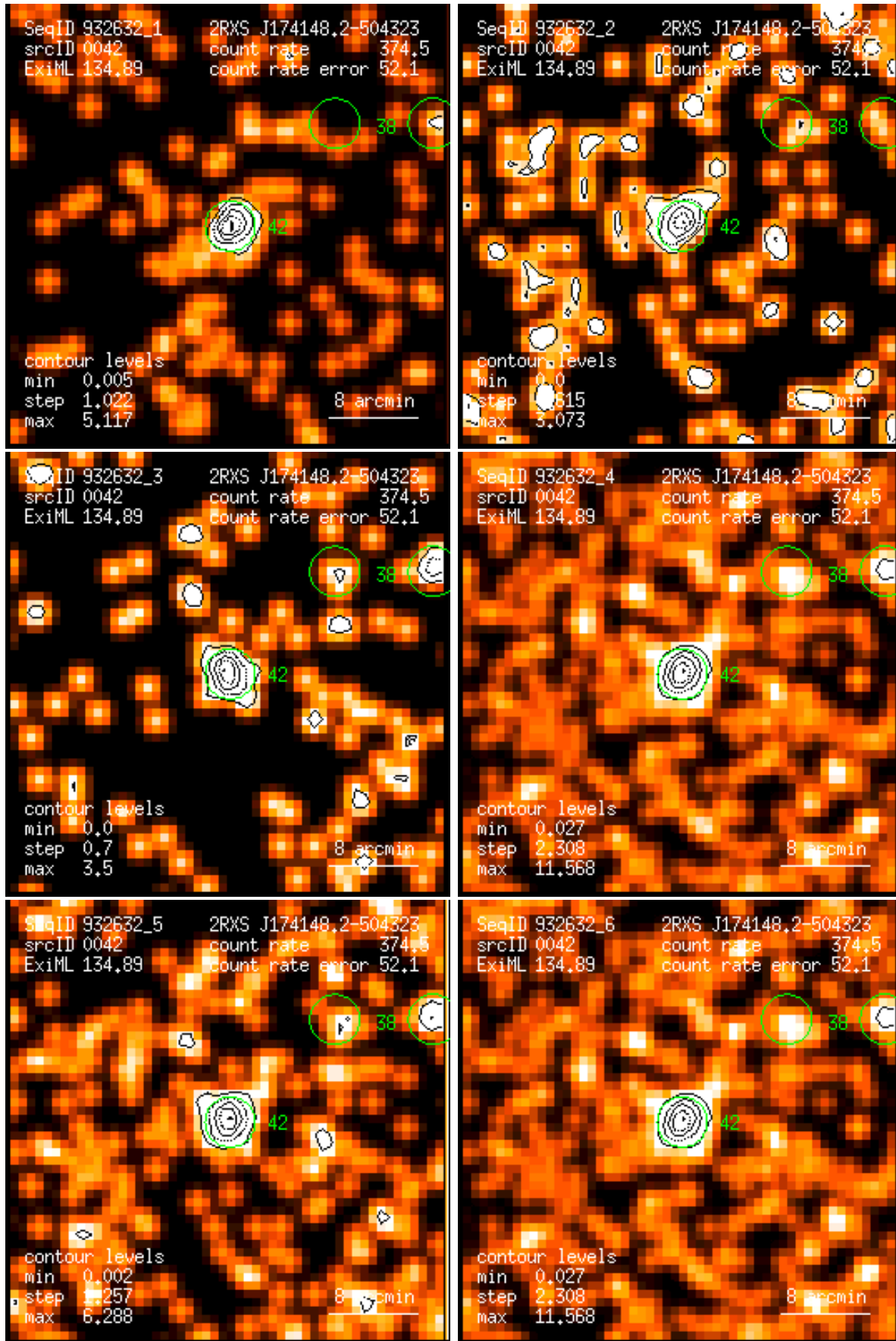
Figure 42: RASS 932632: detection 0042: band rate images, Gaussian filter: (1) PSPC channels 11 – 41, (2) 52 – 90, (3) 91 – 201, (4) 11 – 235, (5) 52 – 201, (6) 11 – 201. Broad band rates in counts/ks. Band rate contour levels in counts/ks/arcmin 2 .
