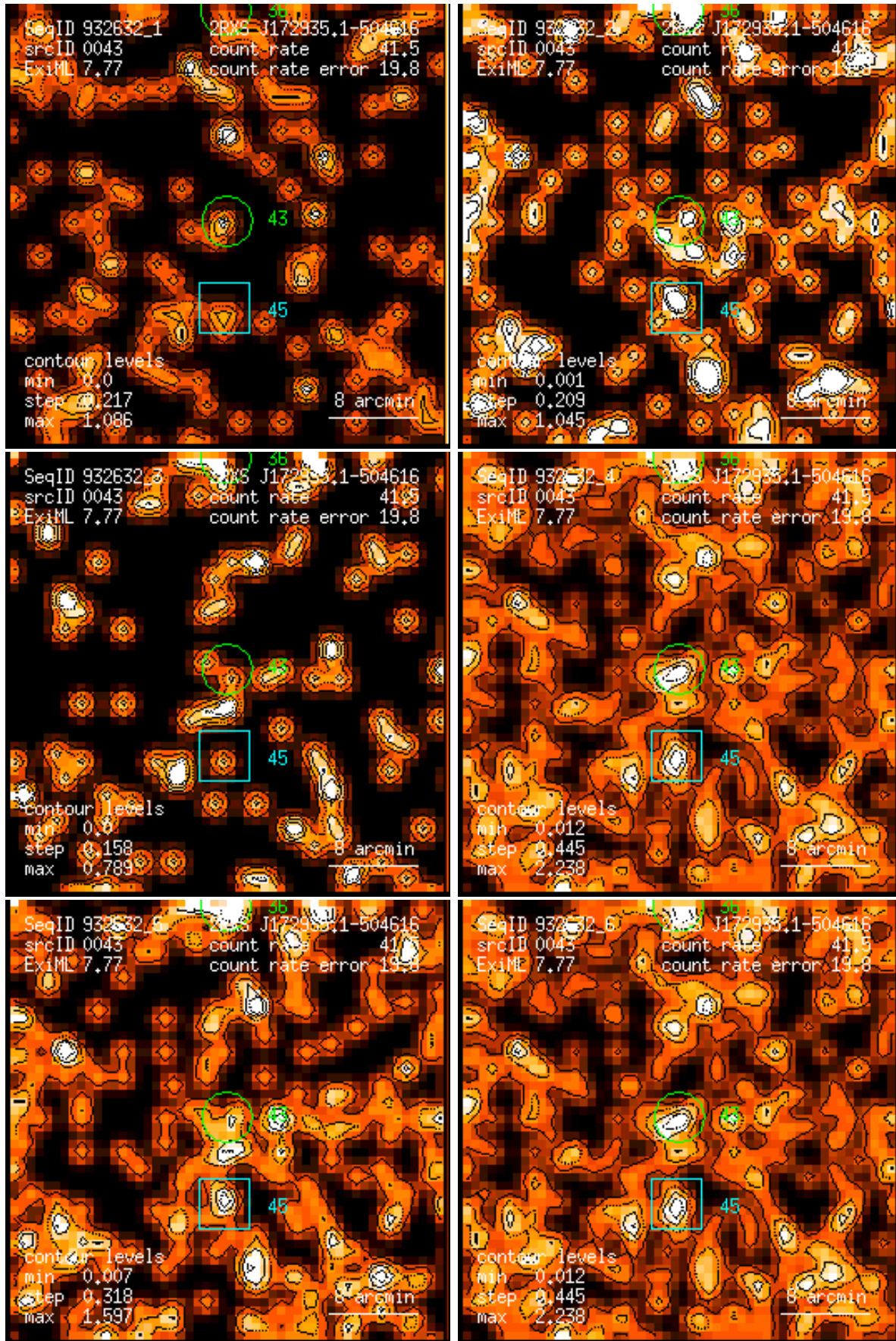
Figure 43: RASS 932632: detection 0043: band rate images, Gaussian filter: (1) PSPC channels 11 – 41, (2) 52 – 90, (3) 91 – 201, (4) 11 – 235, (5) 52 – 201, (6) 11 – 201. Broad band rates in counts/ks. Band rate contour levels in counts/ks/arcmin 2 .
