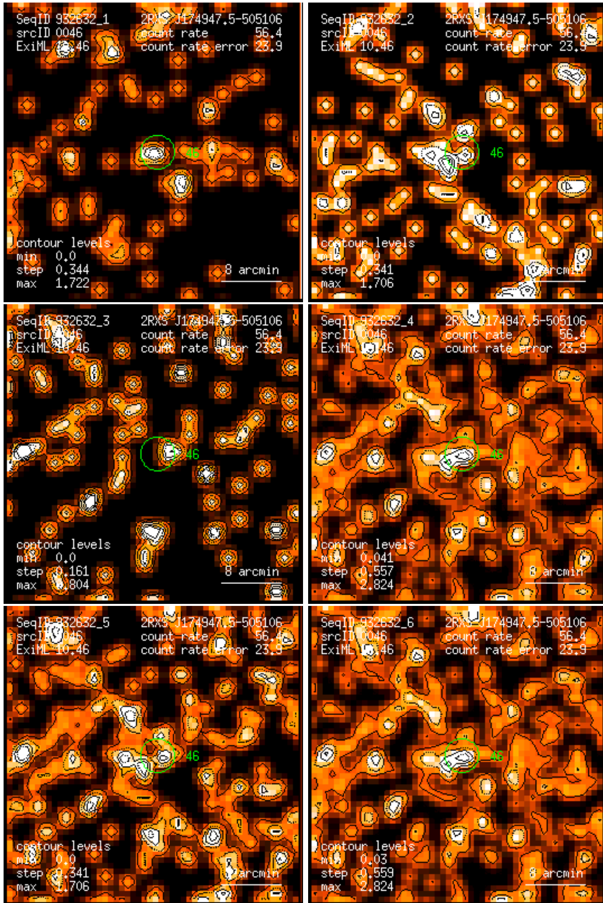
Figure 46: RASS 932632: detection 0046: band rate images, Gaussian filter: (1) PSPC channels 11 – 41, (2) 52 – 90, (3) 91 – 201, (4) 11 – 235, (5) 52 – 201, (6) 11 – 201. Broad band rates in counts/ks. Band rate contour levels in counts/ks/arcmin 2 .
