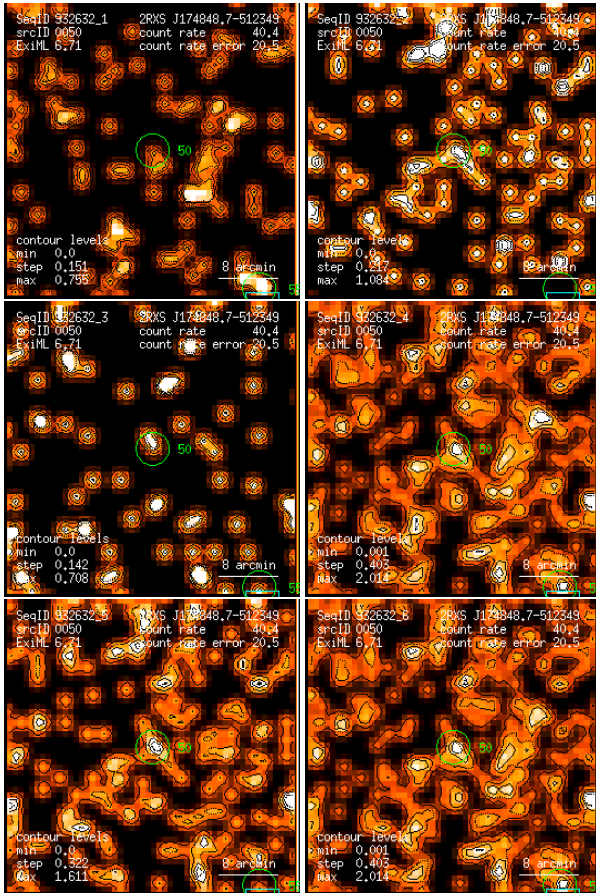
Figure 50: RASS 932632: detection 0050: band rate images, Gaussian filter: (1) PSPC channels 11 – 41, (2) 52 – 90, (3) 91 – 201, (4) 11 – 235, (5) 52 – 201, (6) 11 – 201. Broad band rates in counts/ks. Band rate contour levels in counts/ks/arcmin 2 .
