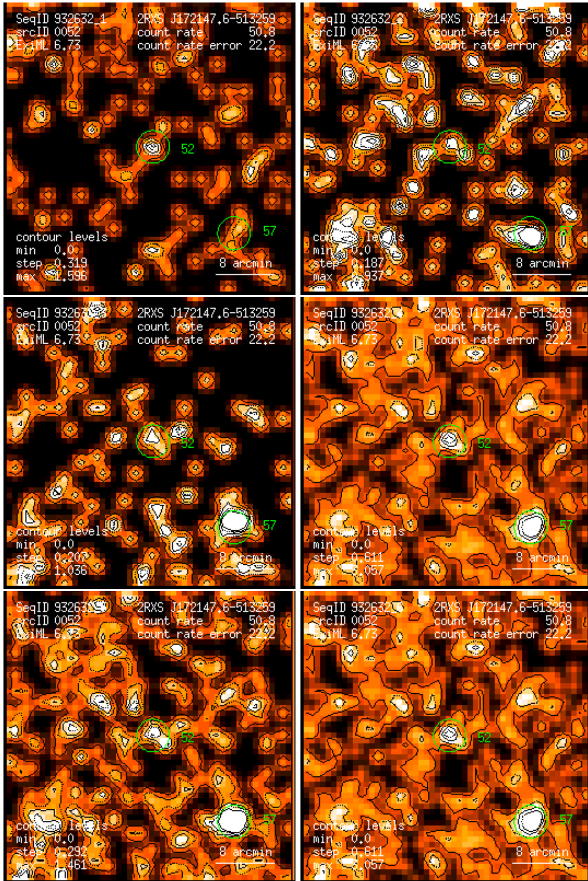
Figure 52: RASS 932632: detection 0052: band rate images, Gaussian filter: (1) PSPC channels 11 – 41, (2) 52 – 90, (3) 91 – 201, (4) 11 – 235, (5) 52 – 201, (6) 11 – 201. Broad band rates in counts/ks. Band rate contour levels in counts/ks/arcmin 2 .
