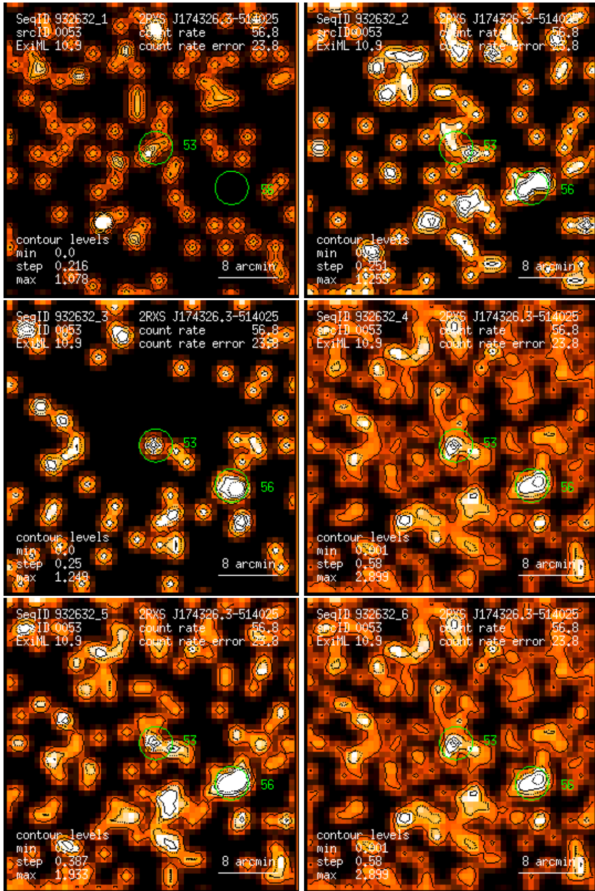
Figure 53: RASS 932632: detection 0053: band rate images, Gaussian filter: (1) PSPC channels 11 – 41, (2) 52 – 90, (3) 91 – 201, (4) 11 – 235, (5) 52 – 201, (6) 11 – 201. Broad band rates in counts/ks. Band rate contour levels in counts/ks/arcmin 2 .
