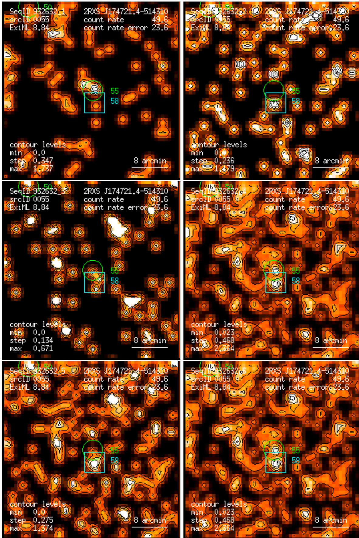
Figure 55: RASS 932632: detection 0055: band rate images, Gaussian filter: (1) PSPC channels 11 – 41, (2) 52 – 90, (3) 91 – 201, (4) 11 – 235, (5) 52 – 201, (6) 11 – 201. Broad band rates in counts/ks. Band rate contour levels in counts/ks/arcmin 2 .
