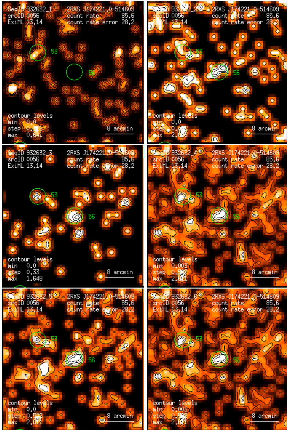
Figure 56: RASS 932632: detection 0056: band rate images, Gaussian filter: (1) PSPC channels 11 – 41, (2) 52 – 90, (3) 91 – 201, (4) 11 – 235, (5) 52 – 201, (6) 11 – 201. Broad band rates in counts/ks. Band rate contour levels in counts/ks/arcmin 2 .
