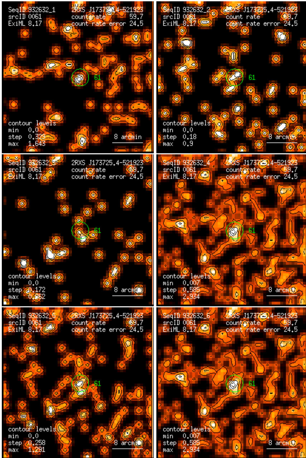
Figure 61: RASS 932632: detection 0061: band rate images, Gaussian filter: (1) PSPC channels 11 – 41, (2) 52 – 90, (3) 91 – 201, (4) 11 – 235, (5) 52 – 201, (6) 11 – 201. Broad band rates in counts/ks. Band rate contour levels in counts/ks/arcmin 2 .
