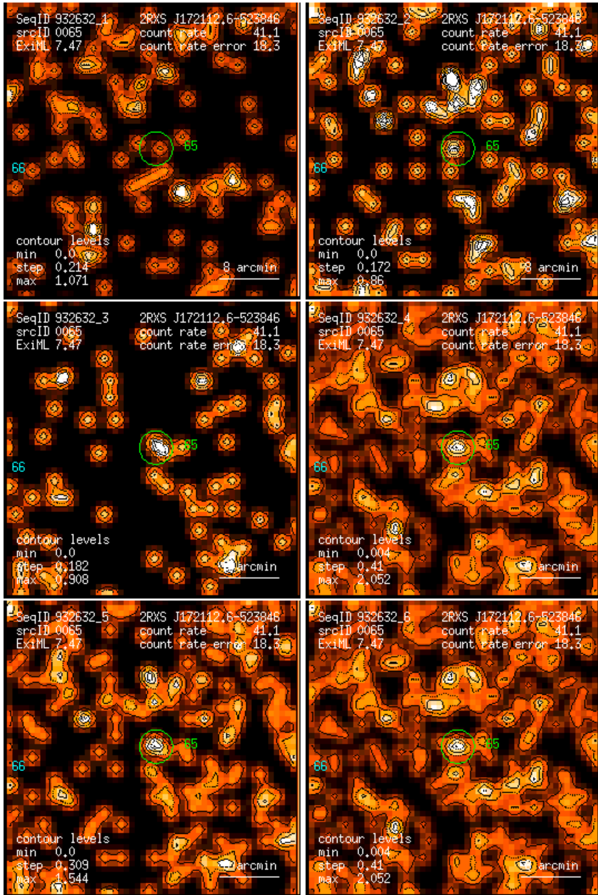
Figure 65: RASS 932632: detection 0065: band rate images, Gaussian filter: (1) PSPC channels 11 – 41, (2) 52 – 90, (3) 91 – 201, (4) 11 – 235, (5) 52 – 201, (6) 11 – 201. Broad band rates in counts/ks. Band rate contour levels in counts/ks/arcmin 2 .
