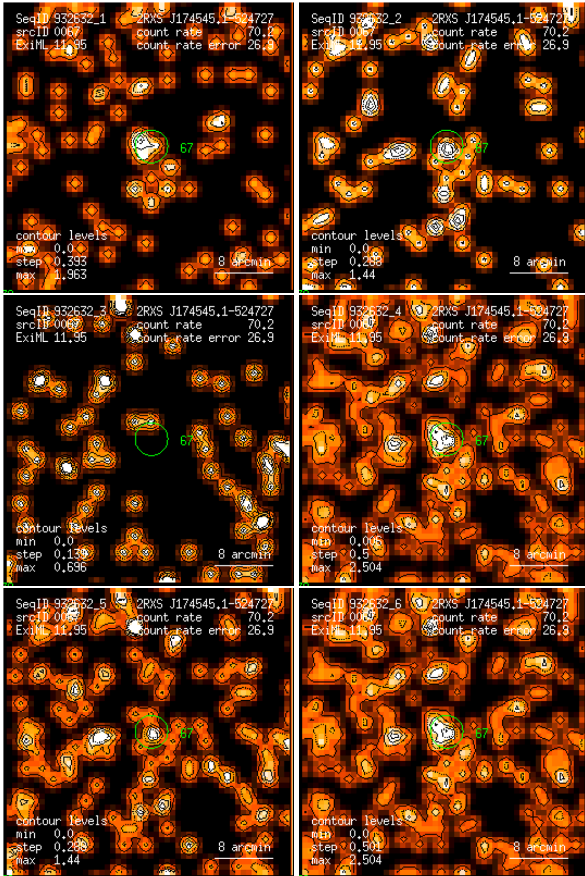
Figure 67: RASS 932632: detection 0067: band rate images, Gaussian filter: (1) PSPC channels 11 – 41, (2) 52 – 90, (3) 91 – 201, (4) 11 – 235, (5) 52 – 201, (6) 11 – 201. Broad band rates in counts/ks. Band rate contour levels in counts/ks/arcmin 2 .
