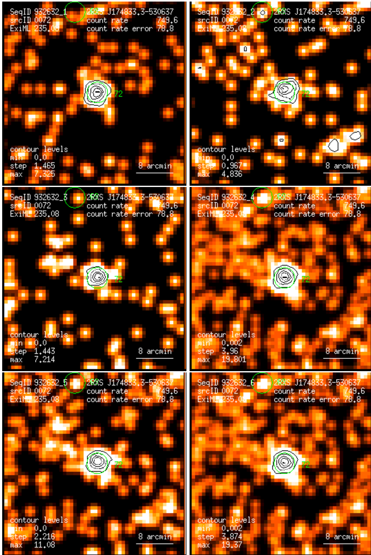
Figure 72: RASS 932632: detection 0072: band rate images, Gaussian filter: (1) PSPC channels 11 – 41, (2) 52 – 90, (3) 91 – 201, (4) 11 – 235, (5) 52 – 201, (6) 11 – 201. Broad band rates in counts/ks. Band rate contour levels in counts/ks/arcmin 2 .
