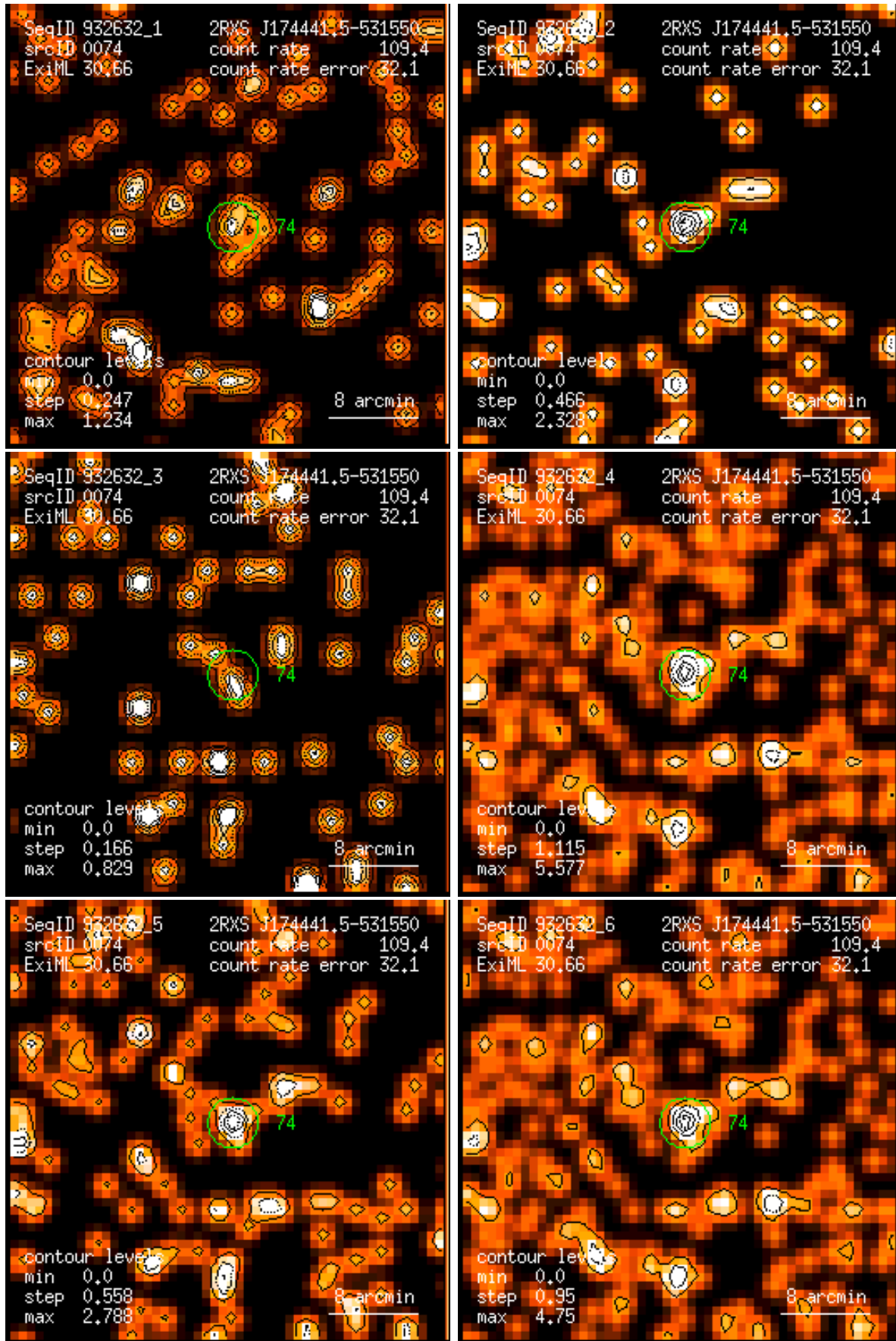
Figure 74: RASS 932632: detection 0074: band rate images, Gaussian filter: (1) PSPC channels 11 – 41, (2) 52 – 90, (3) 91 – 201, (4) 11 – 235, (5) 52 – 201, (6) 11 – 201. Broad band rates in counts/ks. Band rate contour levels in counts/ks/arcmin 2 .
