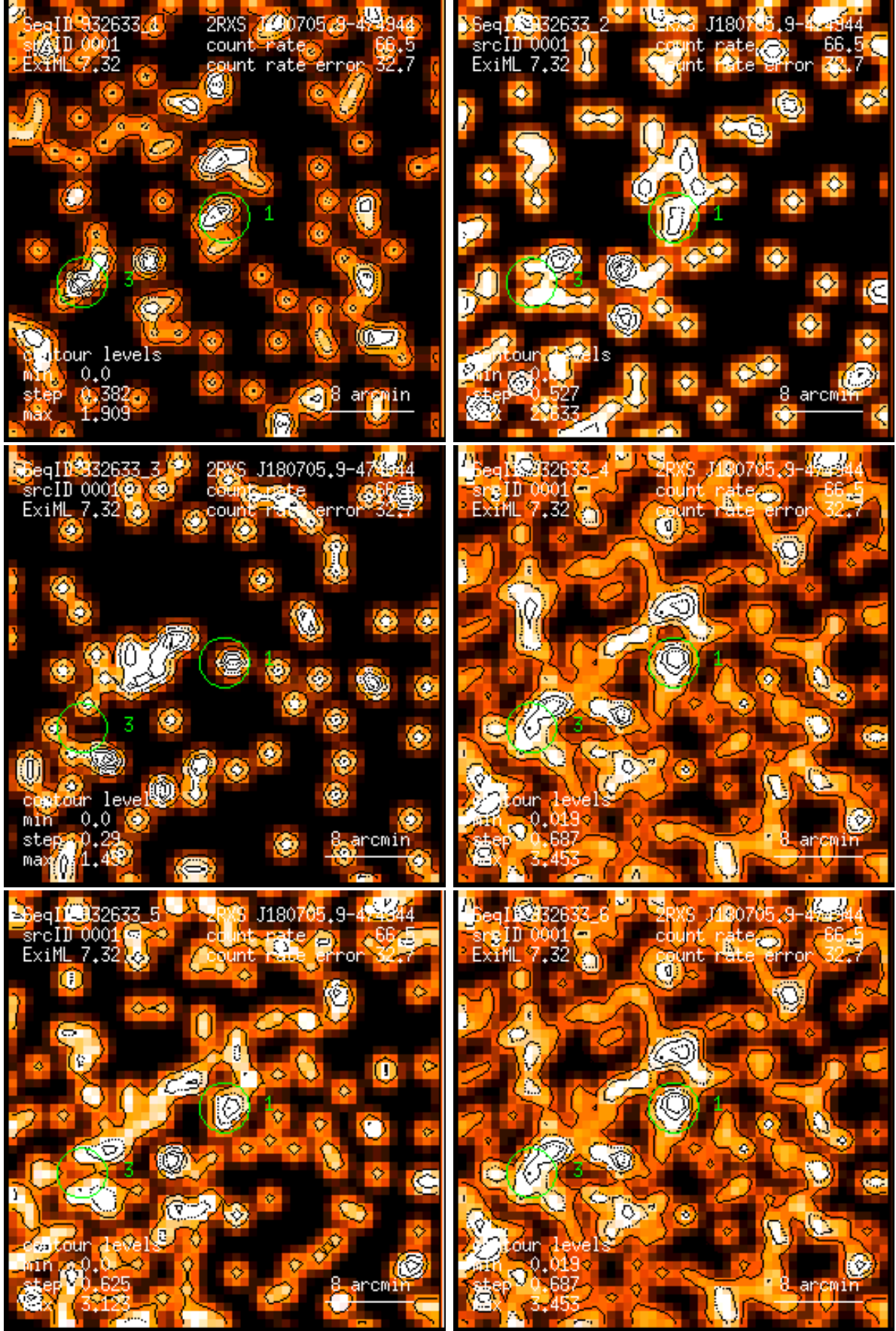
Figure 1: RASS 932633: detection 0001: band rate images, Gaussian filter: (1) PSPC channels 11 – 41, (2) 52 – 90, (3) 91 – 201, (4) 11 – 235, (5) 52 – 201, (6) 11 – 201. Broad band rates in counts/ks. Band rate contour levels in counts/ks/arcmin 2 .
