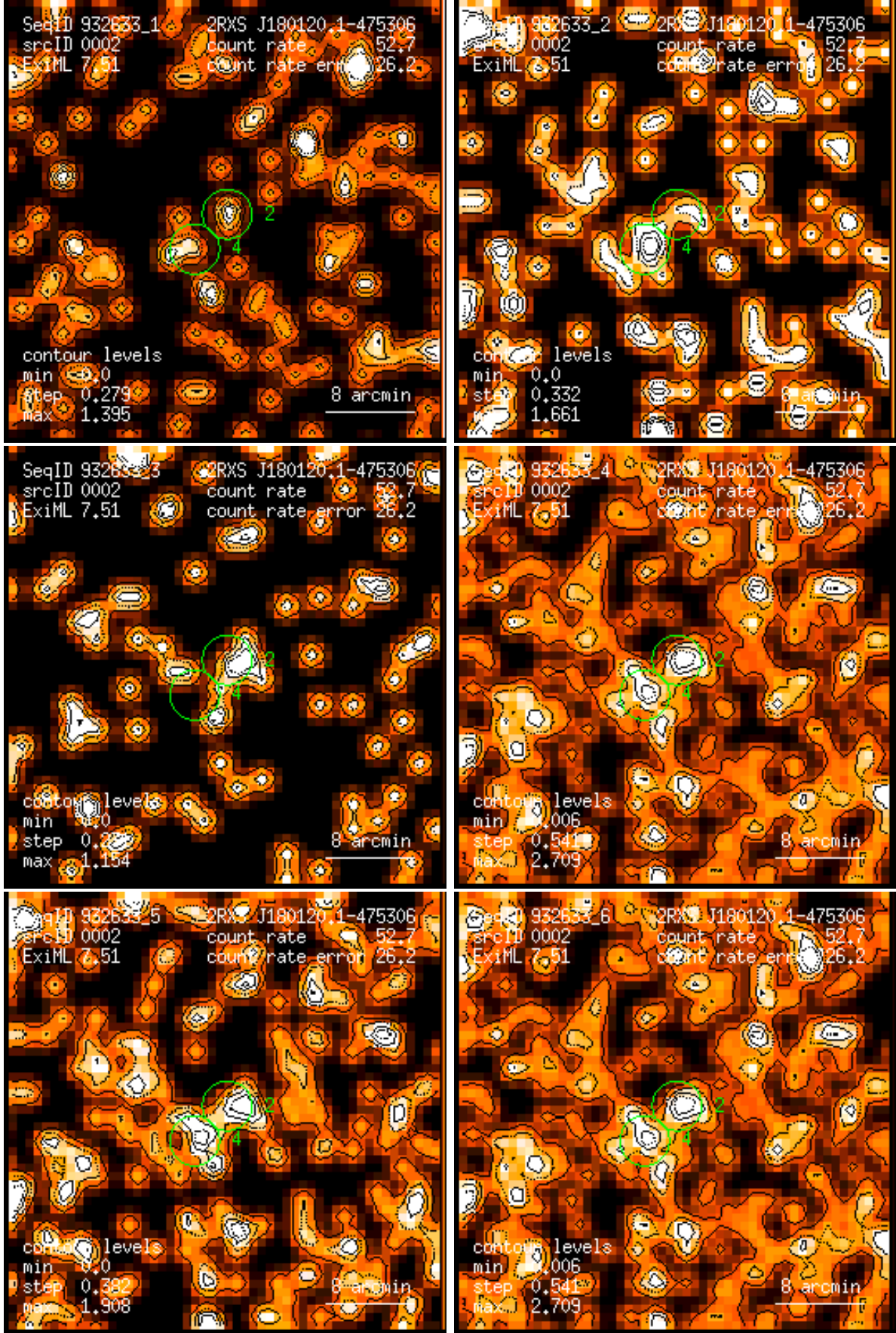
Figure 2: RASS 932633: detection 0002: band rate images, Gaussian filter: (1) PSPC channels 11 – 41, (2) 52 – 90, (3) 91 – 201, (4) 11 – 235, (5) 52 – 201, (6) 11 – 201. Broad band rates in counts/ks. Band rate contour levels in counts/ks/arcmin 2 .
