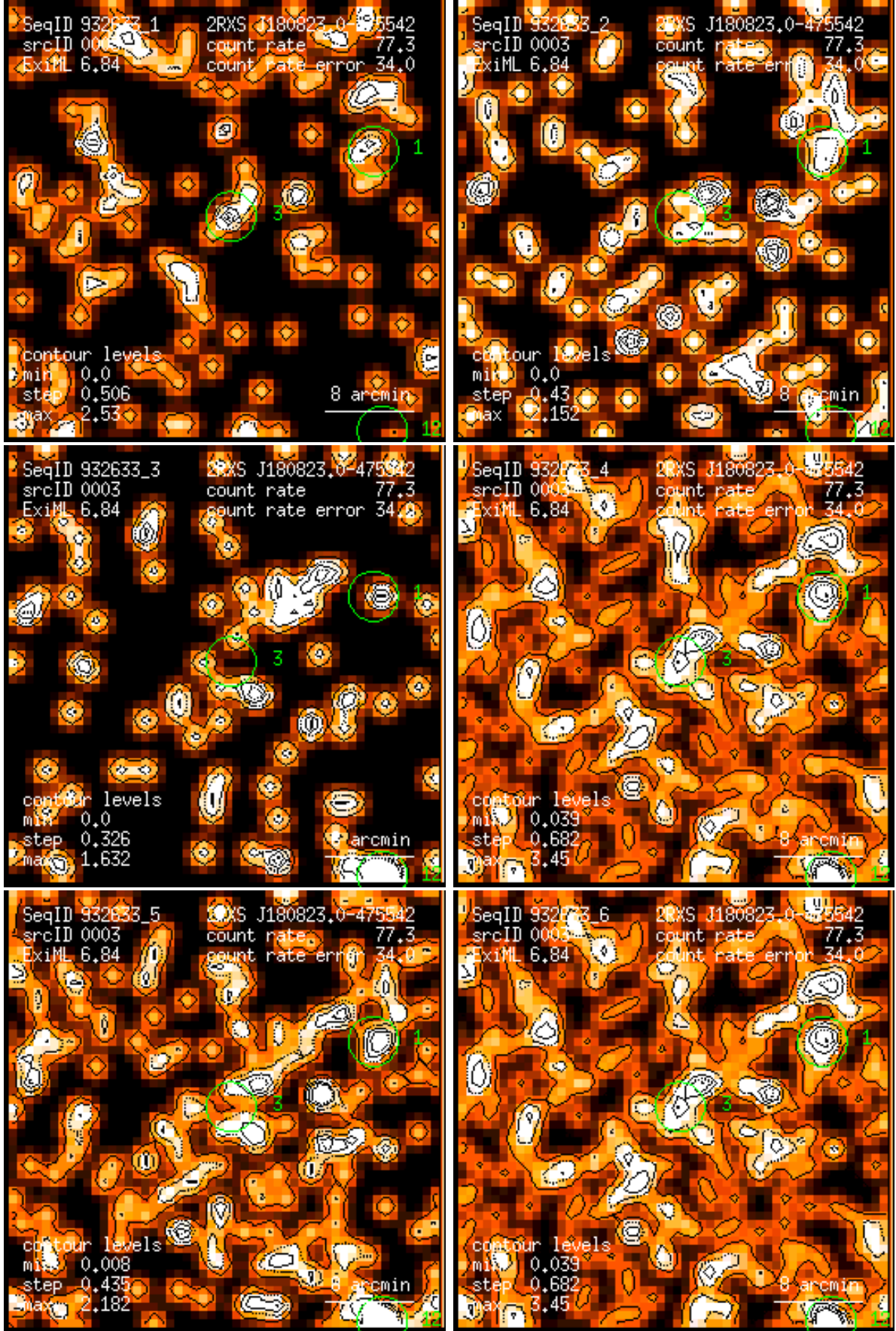
Figure 3: RASS 932633: detection 0003: band rate images, Gaussian filter: (1) PSPC channels 11 – 41, (2) 52 – 90, (3) 91 – 201, (4) 11 – 235, (5) 52 – 201, (6) 11 – 201. Broad band rates in counts/ks. Band rate contour levels in counts/ks/arcmin 2 .
