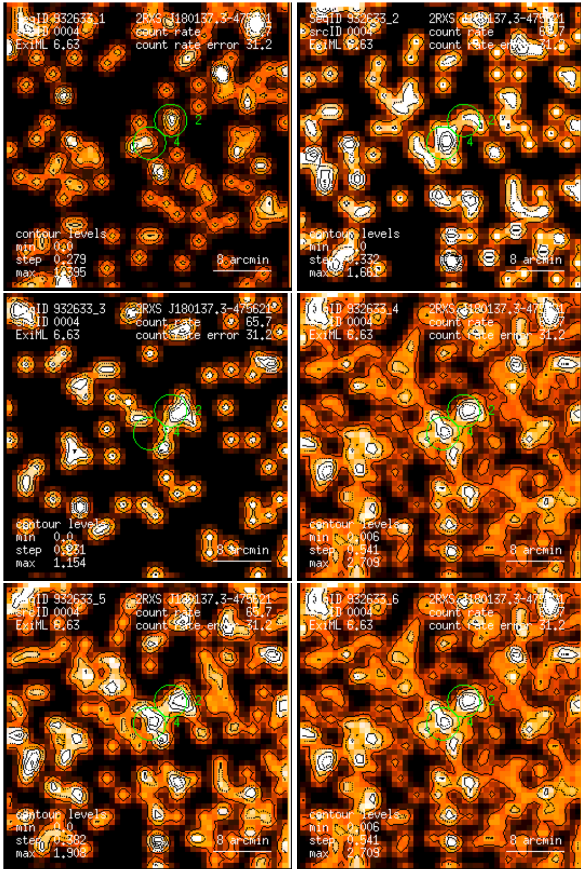
Figure 4: RASS 932633: detection 0004: band rate images, Gaussian filter: (1) PSPC channels 11 – 41, (2) 52 – 90, (3) 91 – 201, (4) 11 – 235, (5) 52 – 201, (6) 11 – 201. Broad band rates in counts/ks. Band rate contour levels in counts/ks/arcmin 2 .
