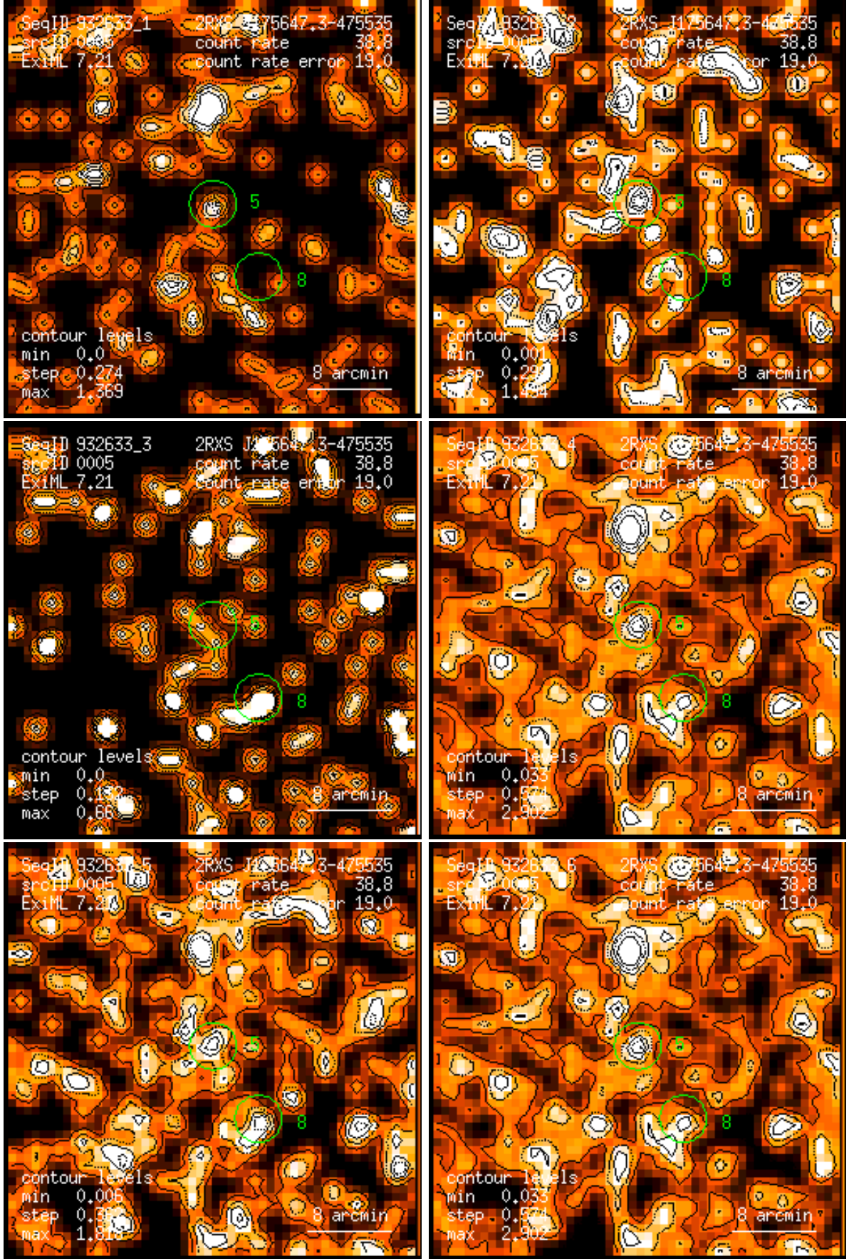
Figure 5: RASS 932633: detection 0005: band rate images, Gaussian filter: (1) PSPC channels 11 – 41, (2) 52 – 90, (3) 91 – 201, (4) 11 – 235, (5) 52 – 201, (6) 11 – 201. Broad band rates in counts/ks. Band rate contour levels in counts/ks/arcmin 2 .
