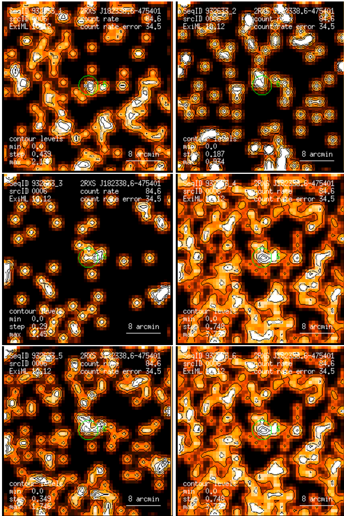
Figure 6: RASS 932633: detection 0006: band rate images, Gaussian filter: (1) PSPC channels 11 – 41, (2) 52 – 90, (3) 91 – 201, (4) 11 – 235, (5) 52 – 201, (6) 11 – 201. Broad band rates in counts/ks. Band rate contour levels in counts/ks/arcmin 2 .
