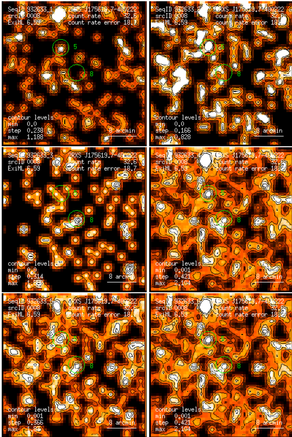
Figure 8: RASS 932633: detection 0008: band rate images, Gaussian filter: (1) PSPC channels 11 – 41, (2) 52 – 90, (3) 91 – 201, (4) 11 – 235, (5) 52 – 201, (6) 11 – 201. Broad band rates in counts/ks. Band rate contour levels in counts/ks/arcmin 2 .
