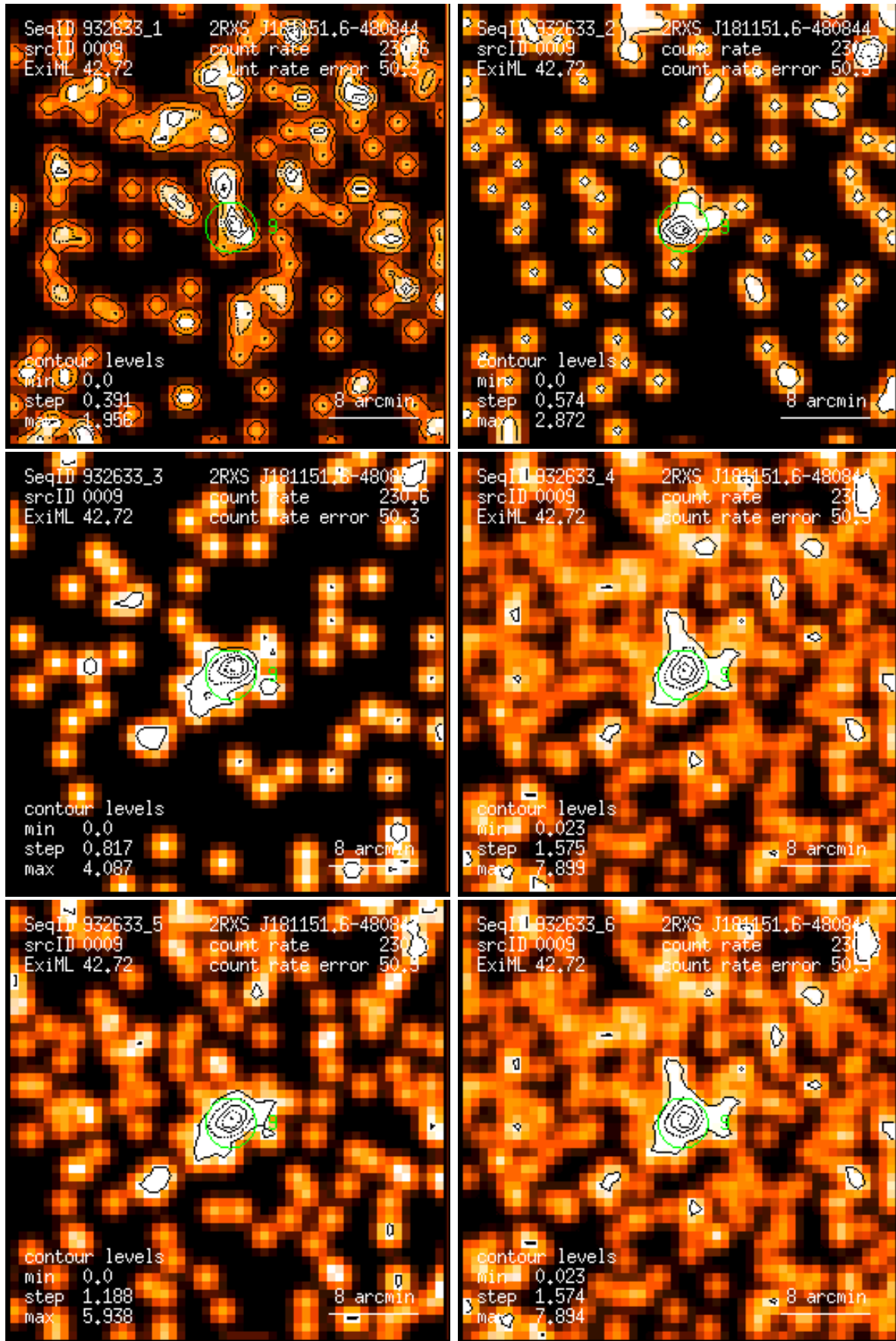
Figure 9: RASS 932633: detection 0009: band rate images, Gaussian filter: (1) PSPC channels 11 – 41, (2) 52 – 90, (3) 91 – 201, (4) 11 – 235, (5) 52 – 201, (6) 11 – 201. Broad band rates in counts/ks. Band rate contour levels in counts/ks/arcmin 2 .
