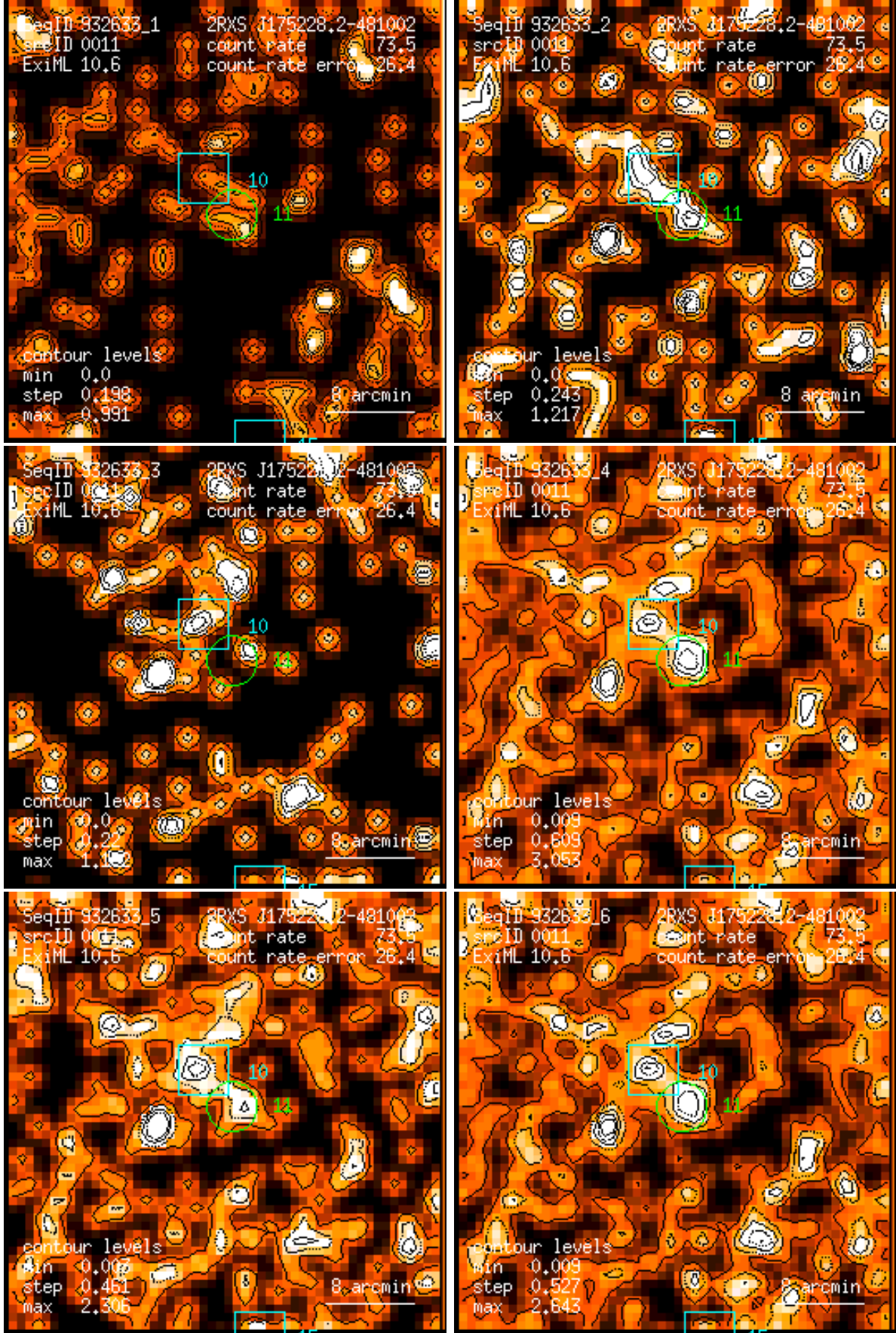
Figure 11: RASS 932633: detection 0011: band rate images, Gaussian filter: (1) PSPC channels 11 – 41, (2) 52 – 90, (3) 91 – 201, (4) 11 – 235, (5) 52 – 201, (6) 11 – 201. Broad band rates in counts/ks. Band rate contour levels in counts/ks/arcmin 2 .
