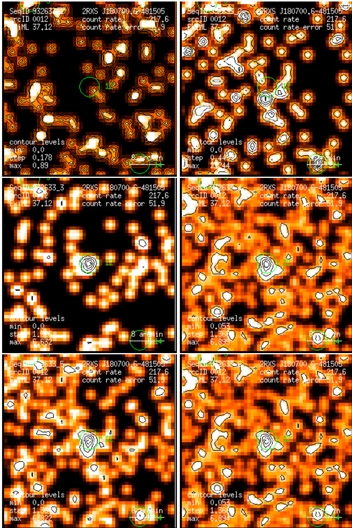
Figure 12: RASS 932633: detection 0012: band rate images, Gaussian filter: (1) PSPC channels 11 – 41, (2) 52 – 90, (3) 91 – 201, (4) 11 – 235, (5) 52 – 201, (6) 11 – 201. Broad band rates in counts/ks. Band rate contour levels in counts/ks/arcmin 2 .
