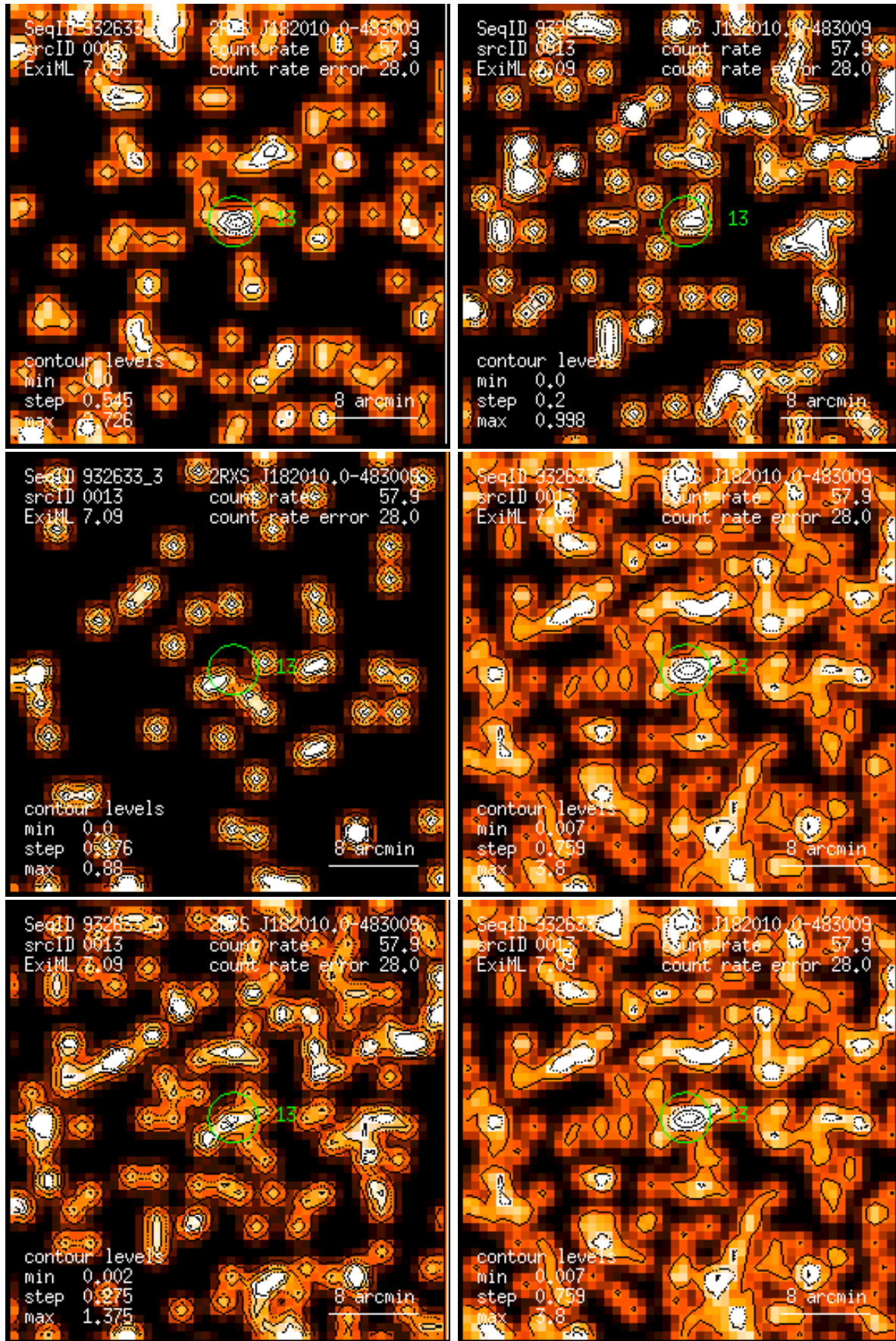
Figure 13: RASS 932633: detection 0013: band rate images, Gaussian filter: (1) PSPC channels 11 – 41, (2) 52 – 90, (3) 91 – 201, (4) 11 – 235, (5) 52 – 201, (6) 11 – 201. Broad band rates in counts/ks. Band rate contour levels in counts/ks/arcmin 2 .
