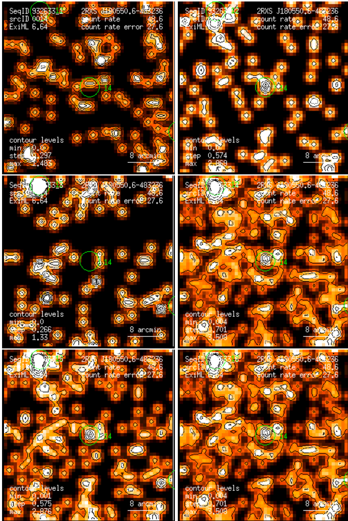
Figure 14: RASS 932633: detection 0014: band rate images, Gaussian filter: (1) PSPC channels 11 – 41, (2) 52 – 90, (3) 91 – 201, (4) 11 – 235, (5) 52 – 201, (6) 11 – 201. Broad band rates in counts/ks. Band rate contour levels in counts/ks/arcmin 2 .
