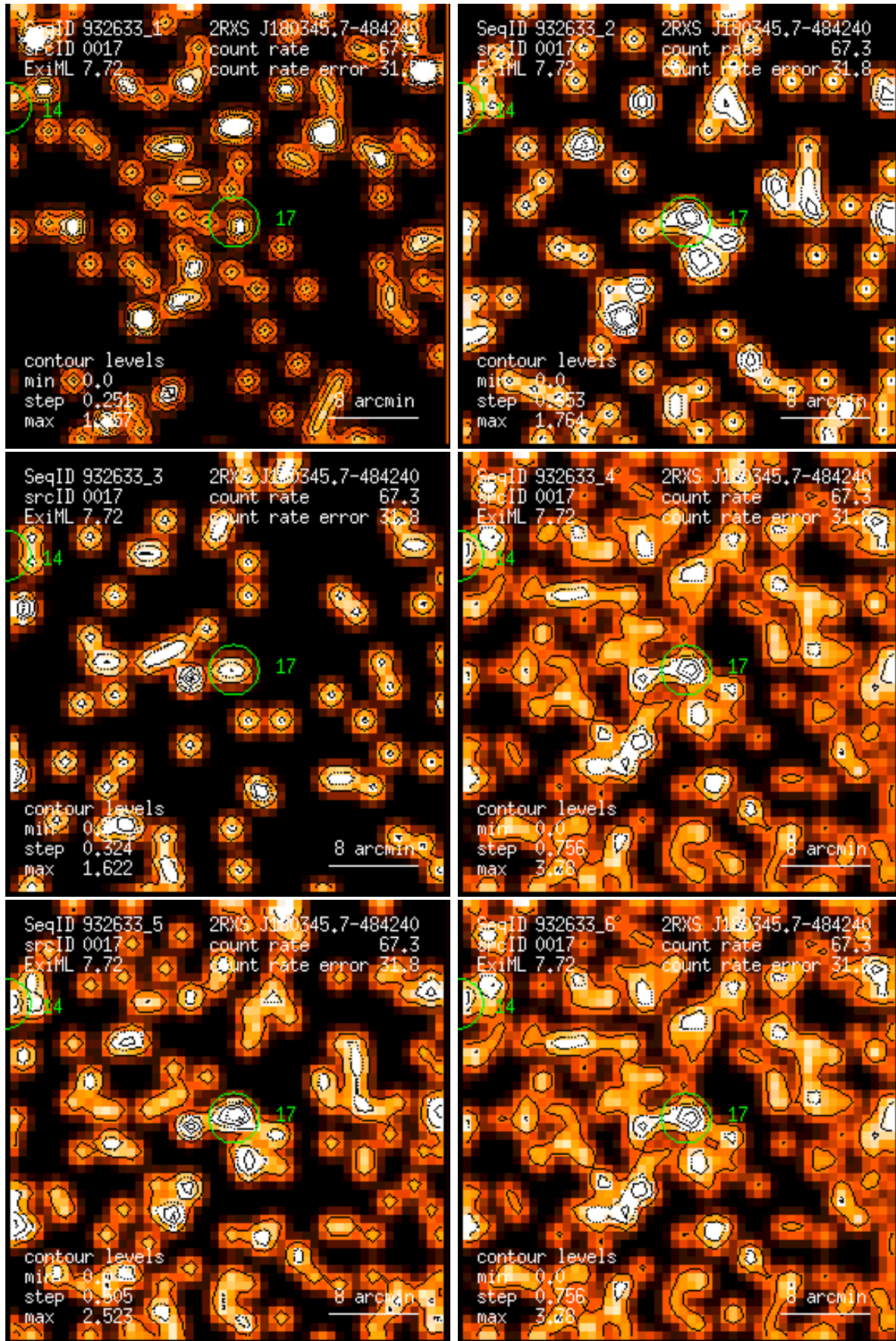
Figure 17: RASS 932633: detection 0017: band rate images, Gaussian filter: (1) PSPC channels 11 – 41, (2) 52 – 90, (3) 91 – 201, (4) 11 – 235, (5) 52 – 201, (6) 11 – 201. Broad band rates in counts/ks. Band rate contour levels in counts/ks/arcmin 2 .
