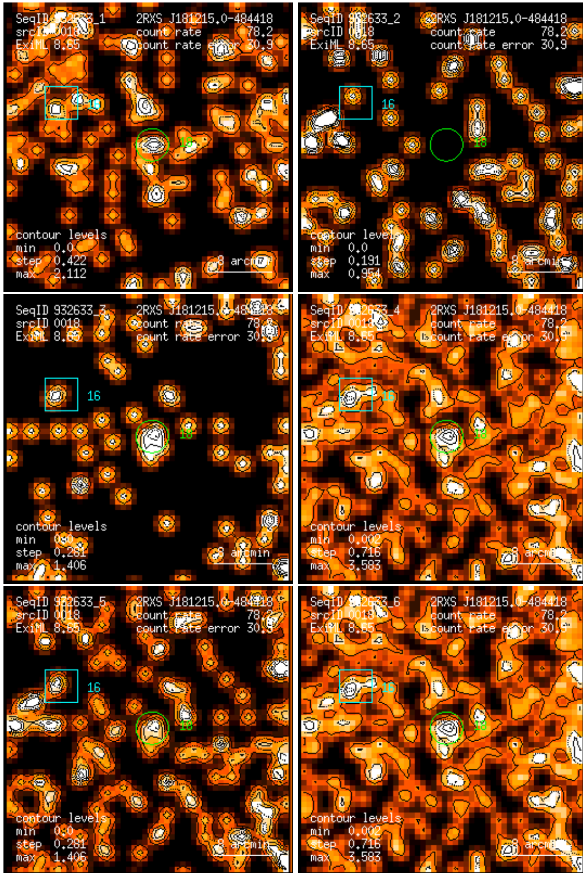
Figure 18: RASS 932633: detection 0018: band rate images, Gaussian filter: (1) PSPC channels 11 – 41, (2) 52 – 90, (3) 91 – 201, (4) 11 – 235, (5) 52 – 201, (6) 11 – 201. Broad band rates in counts/ks. Band rate contour levels in counts/ks/arcmin 2 .
