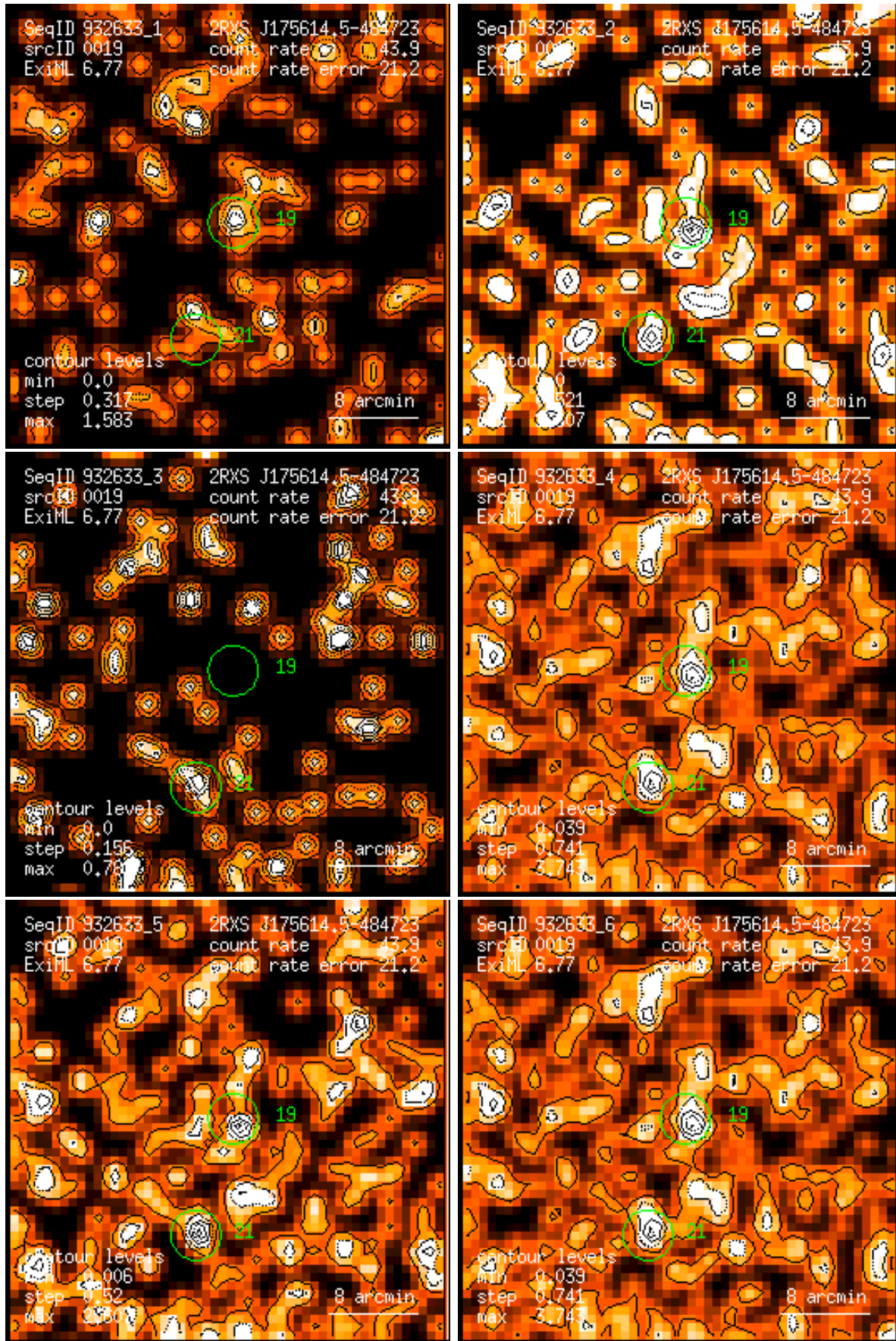
Figure 19: RASS 932633: detection 0019: band rate images, Gaussian filter: (1) PSPC channels 11 – 41, (2) 52 – 90, (3) 91 – 201, (4) 11 – 235, (5) 52 – 201, (6) 11 – 201. Broad band rates in counts/ks. Band rate contour levels in counts/ks/arcmin 2 .
