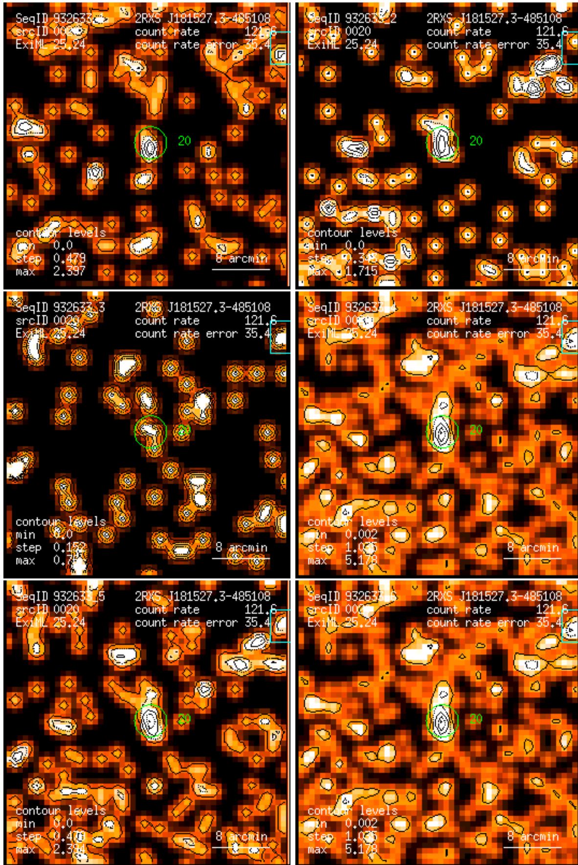
Figure 20: RASS 932633: detection 0020: band rate images, Gaussian filter: (1) PSPC channels 11 – 41, (2) 52 – 90, (3) 91 – 201, (4) 11 – 235, (5) 52 – 201, (6) 11 – 201. Broad band rates in counts/ks. Band rate contour levels in counts/ks/arcmin 2 .
