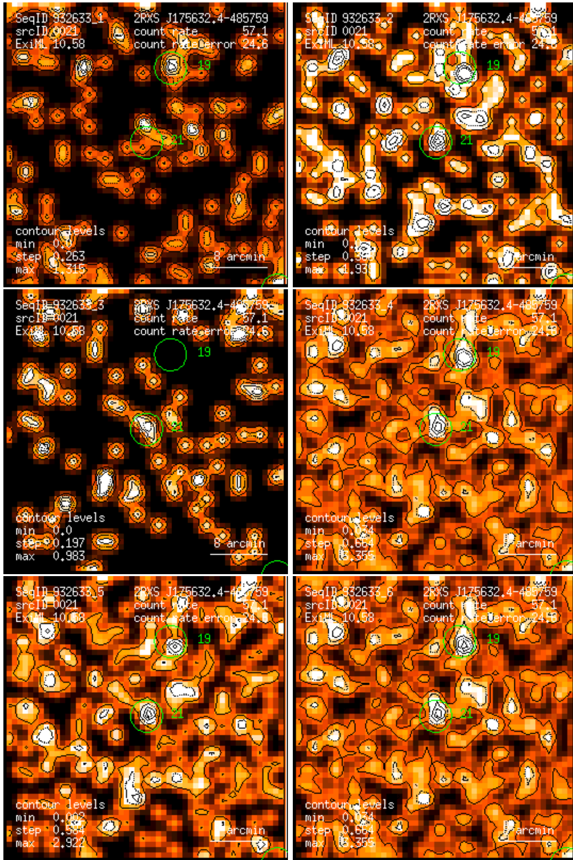
Figure 21: RASS 932633: detection 0021: band rate images, Gaussian filter: (1) PSPC channels 11 – 41, (2) 52 – 90, (3) 91 – 201, (4) 11 – 235, (5) 52 – 201, (6) 11 – 201. Broad band rates in counts/ks. Band rate contour levels in counts/ks/arcmin 2 .
