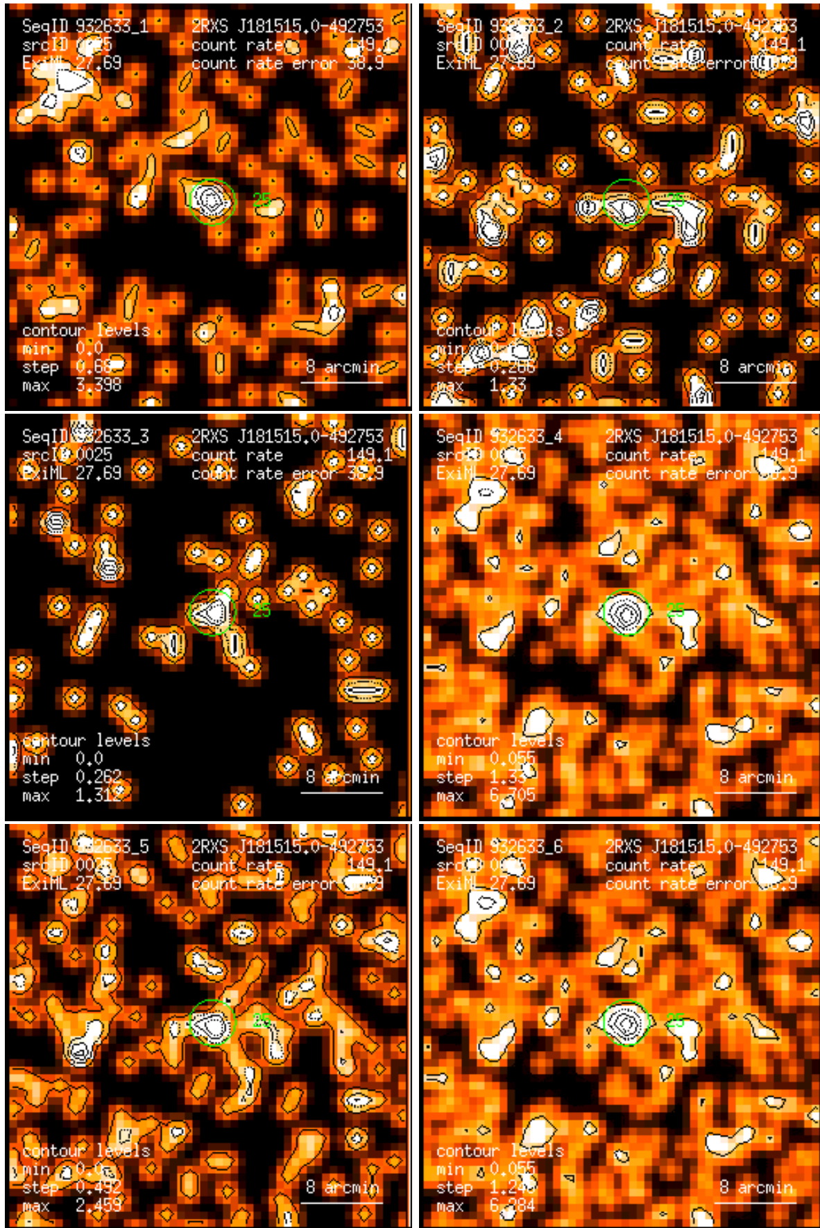
Figure 25: RASS 932633: detection 0025: band rate images, Gaussian filter: (1) PSPC channels 11 – 41, (2) 52 – 90, (3) 91 – 201, (4) 11 – 235, (5) 52 – 201, (6) 11 – 201. Broad band rates in counts/ks. Band rate contour levels in counts/ks/arcmin 2 .
