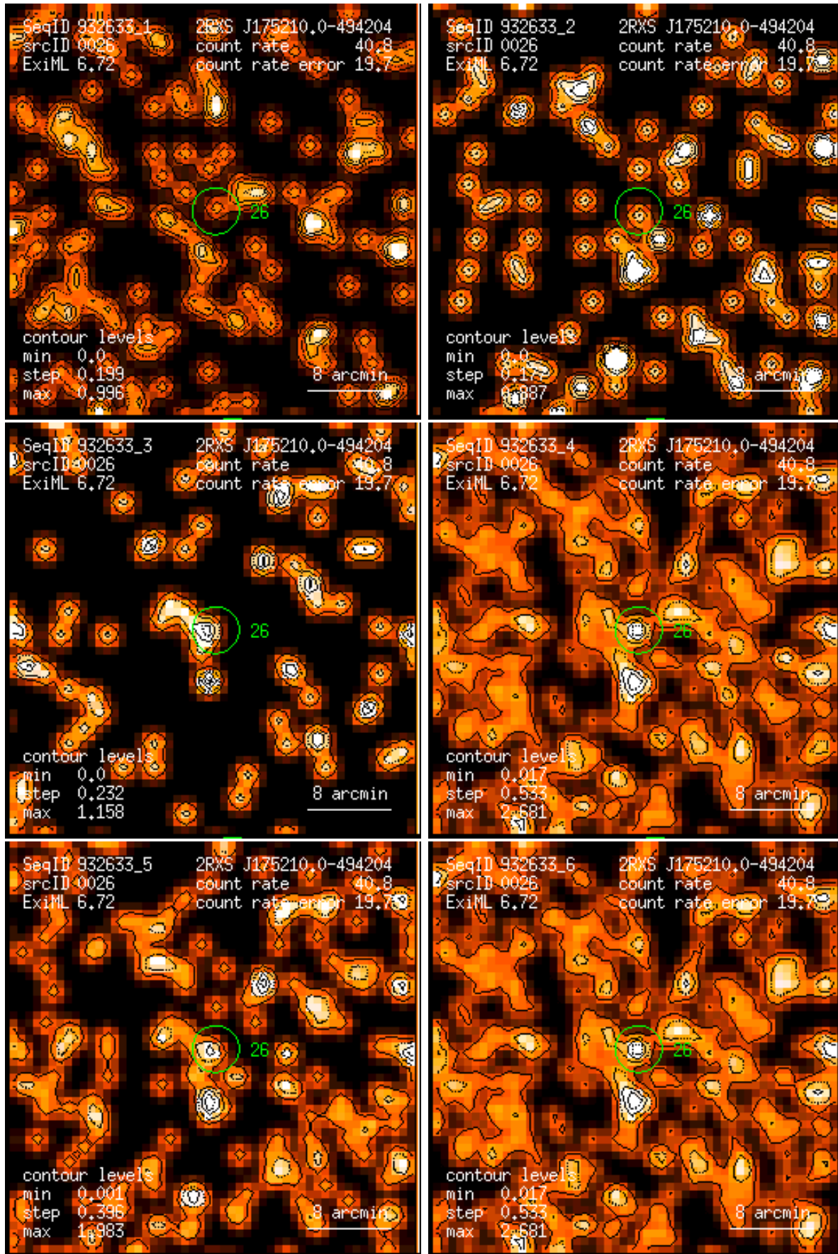
Figure 26: RASS 932633: detection 0026: band rate images, Gaussian filter: (1) PSPC channels 11 – 41, (2) 52 – 90, (3) 91 – 201, (4) 11 – 235, (5) 52 – 201, (6) 11 – 201. Broad band rates in counts/ks. Band rate contour levels in counts/ks/arcmin 2 .
