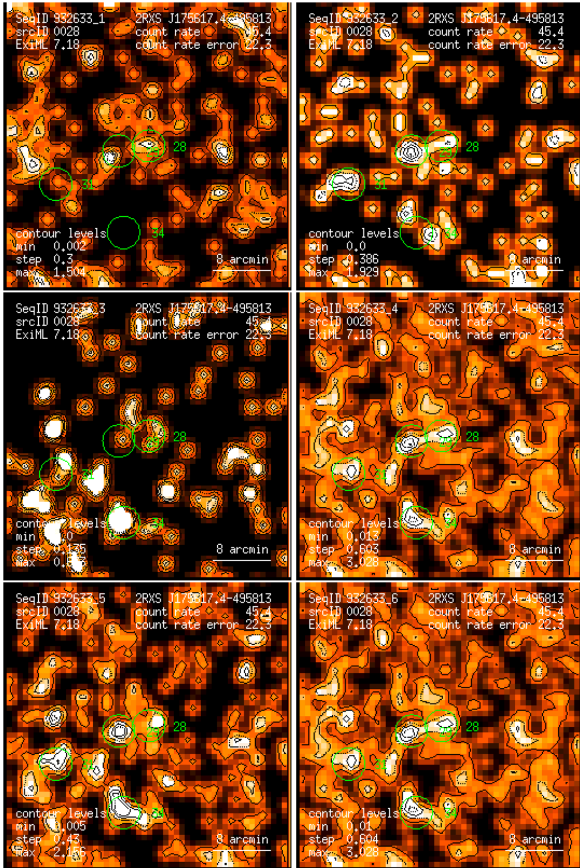
Figure 28: RASS 932633: detection 0028: band rate images, Gaussian filter: (1) PSPC channels 11 – 41, (2) 52 – 90, (3) 91 – 201, (4) 11 – 235, (5) 52 – 201, (6) 11 – 201. Broad band rates in counts/ks. Band rate contour levels in counts/ks/arcmin 2 .
