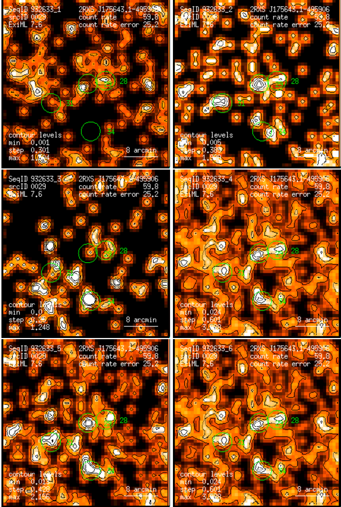
Figure 29: RASS 932633: detection 0029: band rate images, Gaussian filter: (1) PSPC channels 11 – 41, (2) 52 – 90, (3) 91 – 201, (4) 11 – 235, (5) 52 – 201, (6) 11 – 201. Broad band rates in counts/ks. Band rate contour levels in counts/ks/arcmin 2 .
