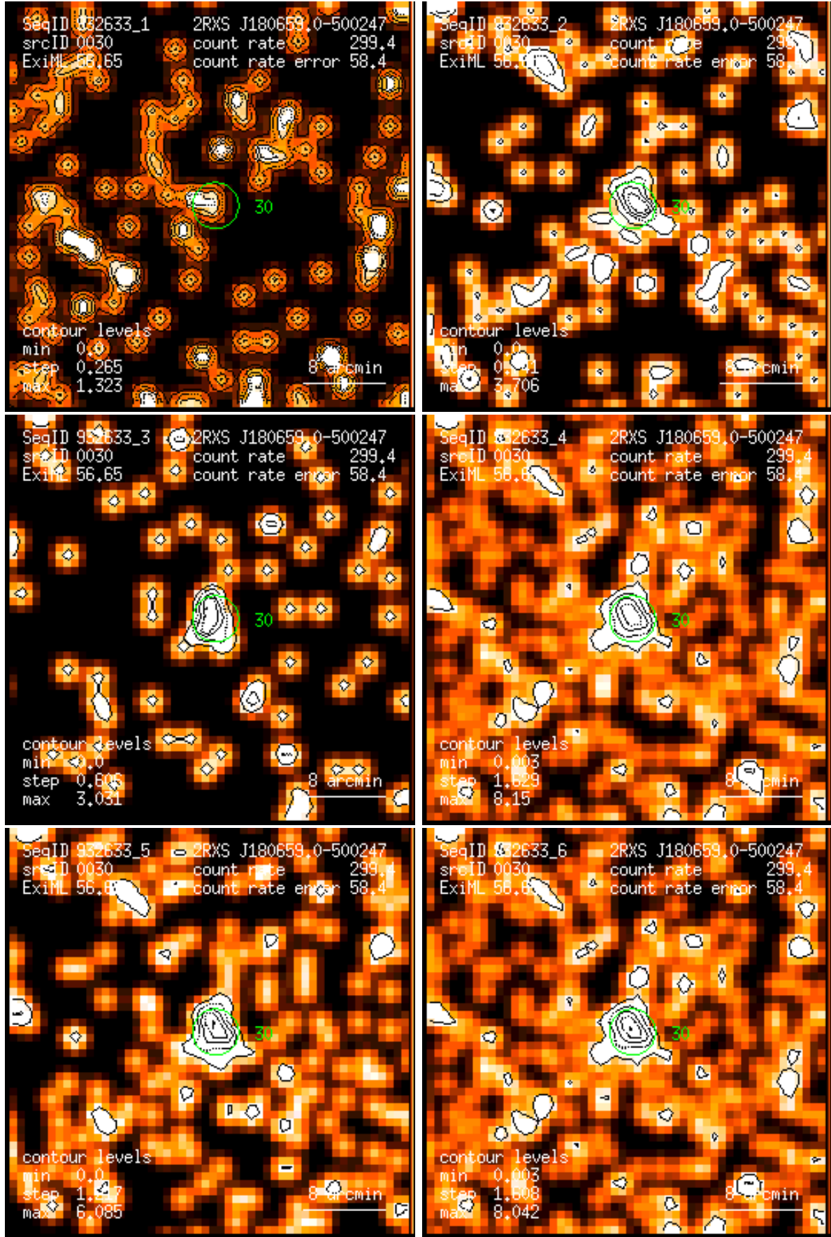
Figure 30: RASS 932633: detection 0030: band rate images, Gaussian filter: (1) PSPC channels 11 – 41, (2) 52 – 90, (3) 91 – 201, (4) 11 – 235, (5) 52 – 201, (6) 11 – 201. Broad band rates in counts/ks. Band rate contour levels in counts/ks/arcmin 2 .
