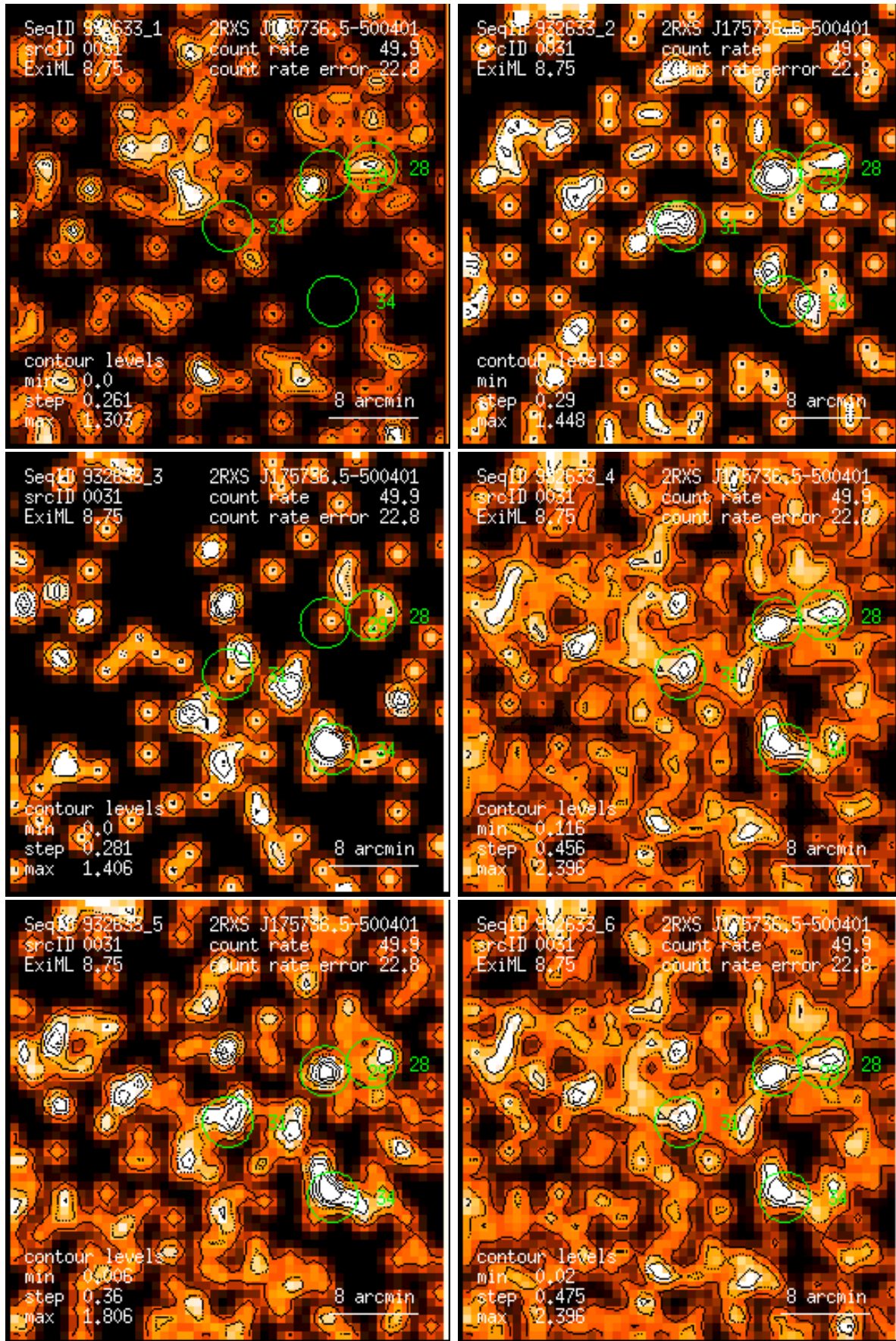
Figure 31: RASS 932633: detection 0031: band rate images, Gaussian filter: (1) PSPC channels 11 – 41, (2) 52 – 90, (3) 91 – 201, (4) 11 – 235, (5) 52 – 201, (6) 11 – 201. Broad band rates in counts/ks. Band rate contour levels in counts/ks/arcmin 2 .
