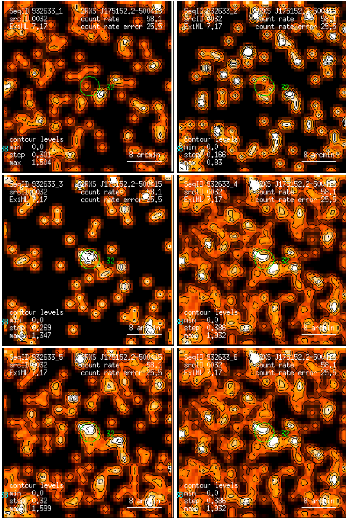
Figure 32: RASS 932633: detection 0032: band rate images, Gaussian filter: (1) PSPC channels 11 – 41, (2) 52 – 90, (3) 91 – 201, (4) 11 – 235, (5) 52 – 201, (6) 11 – 201. Broad band rates in counts/ks. Band rate contour levels in counts/ks/arcmin 2 .
