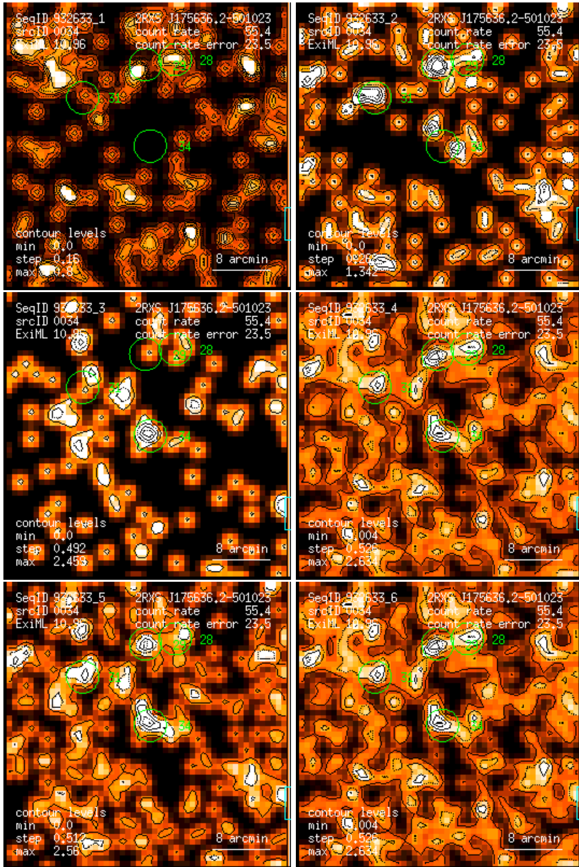
Figure 34: RASS 932633: detection 0034: band rate images, Gaussian filter: (1) PSPC channels 11 – 41, (2) 52 – 90, (3) 91 – 201, (4) 11 – 235, (5) 52 – 201, (6) 11 – 201. Broad band rates in counts/ks. Band rate contour levels in counts/ks/arcmin 2 .
