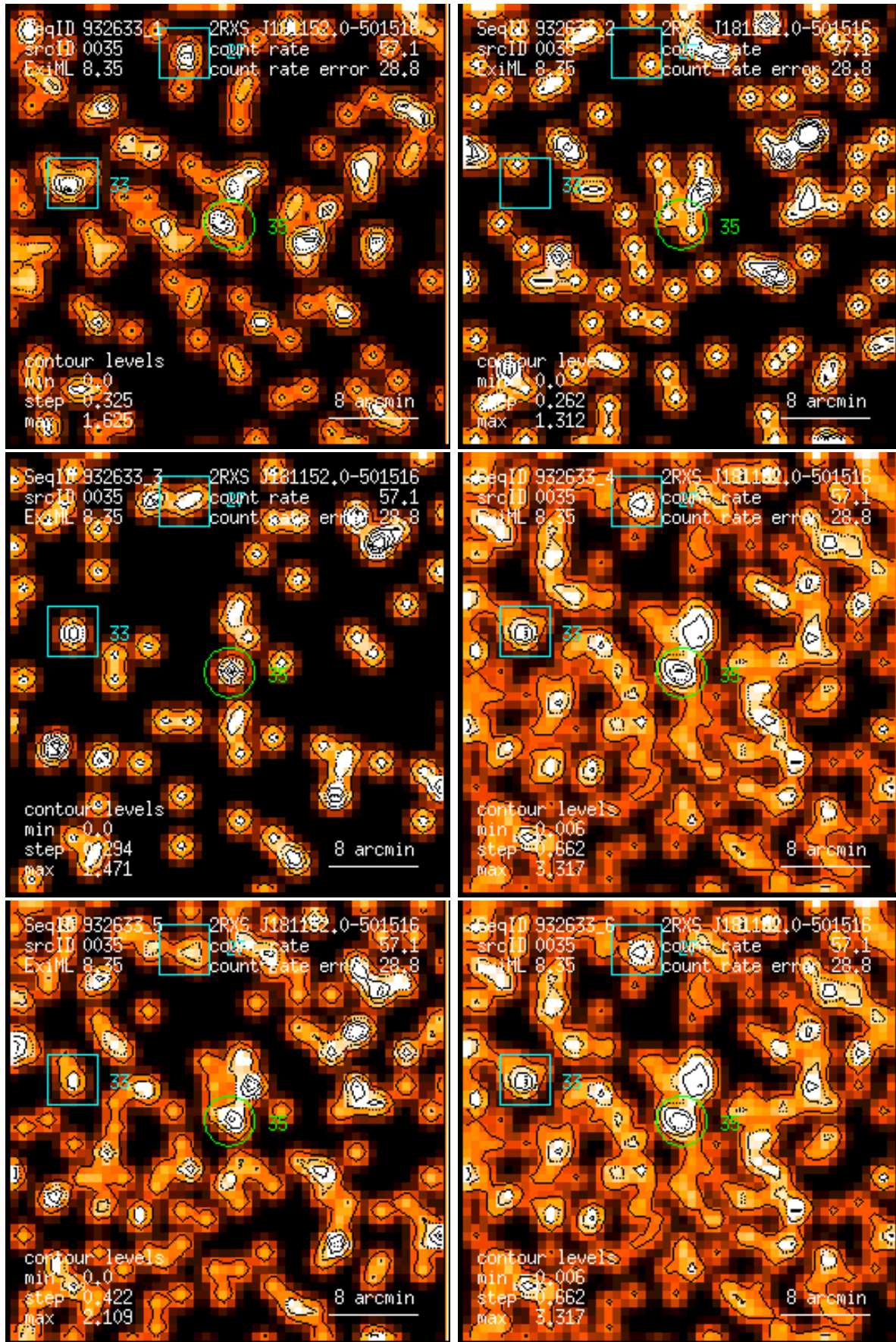
Figure 35: RASS 932633: detection 0035: band rate images, Gaussian filter: (1) PSPC channels 11 – 41, (2) 52 – 90, (3) 91 – 201, (4) 11 – 235, (5) 52 – 201, (6) 11 – 201. Broad band rates in counts/ks. Band rate contour levels in counts/ks/arcmin 2 .
