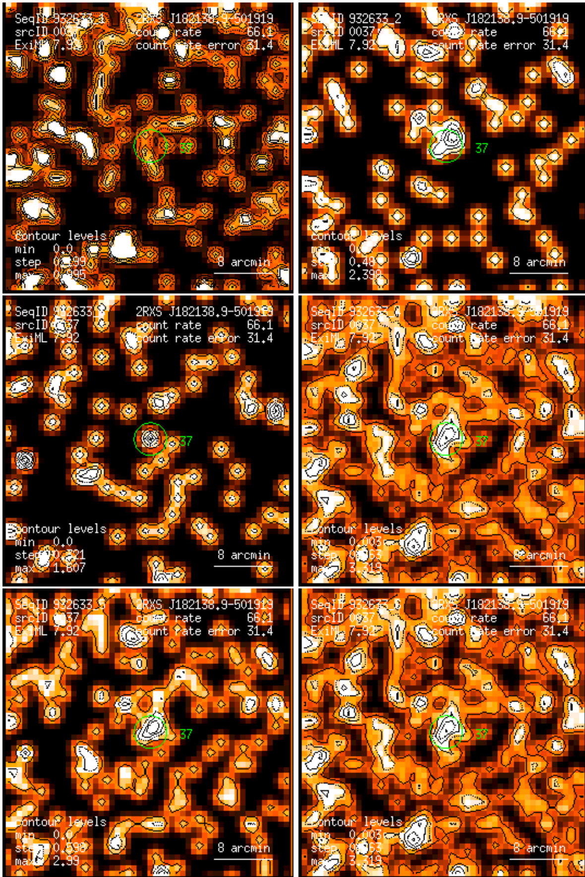
Figure 37: RASS 932633: detection 0037: band rate images, Gaussian filter: (1) PSPC channels 11 – 41, (2) 52 – 90, (3) 91 – 201, (4) 11 – 235, (5) 52 – 201, (6) 11 – 201. Broad band rates in counts/ks. Band rate contour levels in counts/ks/arcmin 2 .
