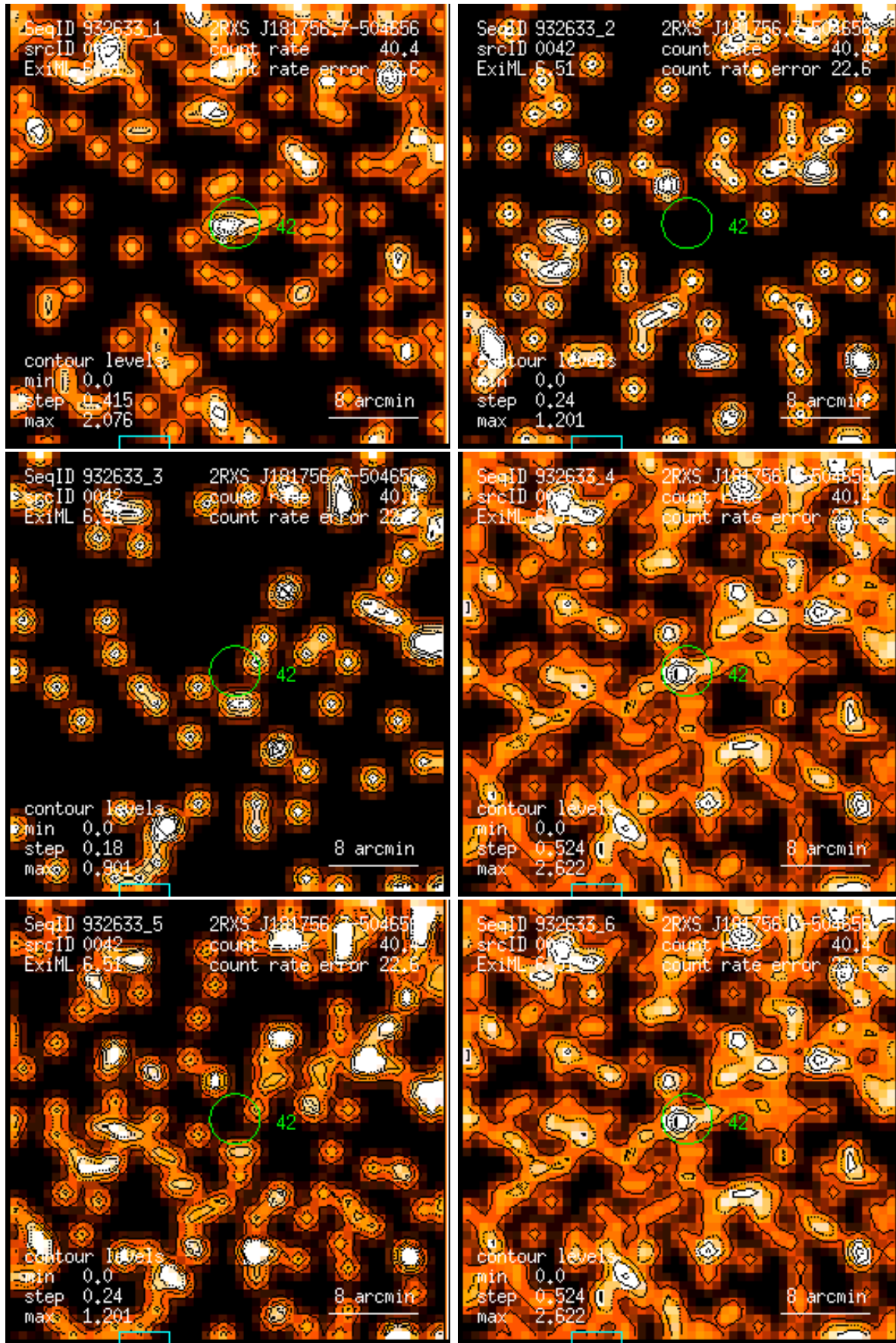
Figure 42: RASS 932633: detection 0042: band rate images, Gaussian filter: (1) PSPC channels 11 – 41, (2) 52 – 90, (3) 91 – 201, (4) 11 – 235, (5) 52 – 201, (6) 11 – 201. Broad band rates in counts/ks. Band rate contour levels in counts/ks/arcmin 2 .
