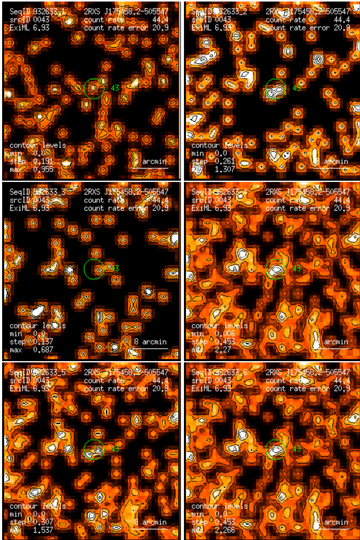
Figure 43: RASS 932633: detection 0043: band rate images, Gaussian filter: (1) PSPC channels 11 – 41, (2) 52 – 90, (3) 91 – 201, (4) 11 – 235, (5) 52 – 201, (6) 11 – 201. Broad band rates in counts/ks. Band rate contour levels in counts/ks/arcmin 2 .
