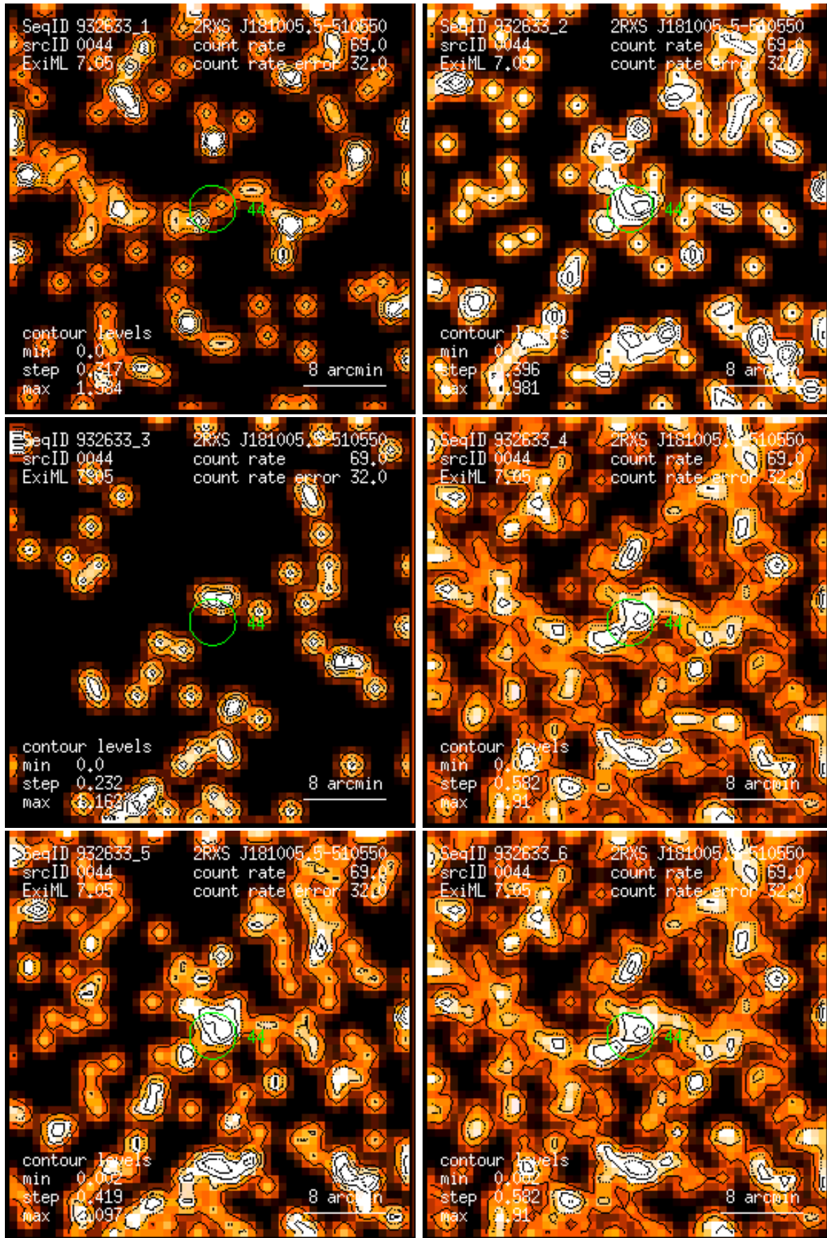
Figure 44: RASS 932633: detection 0044: band rate images, Gaussian filter: (1) PSPC channels 11 – 41, (2) 52 – 90, (3) 91 – 201, (4) 11 – 235, (5) 52 – 201, (6) 11 – 201. Broad band rates in counts/ks. Band rate contour levels in counts/ks/arcmin 2 .
