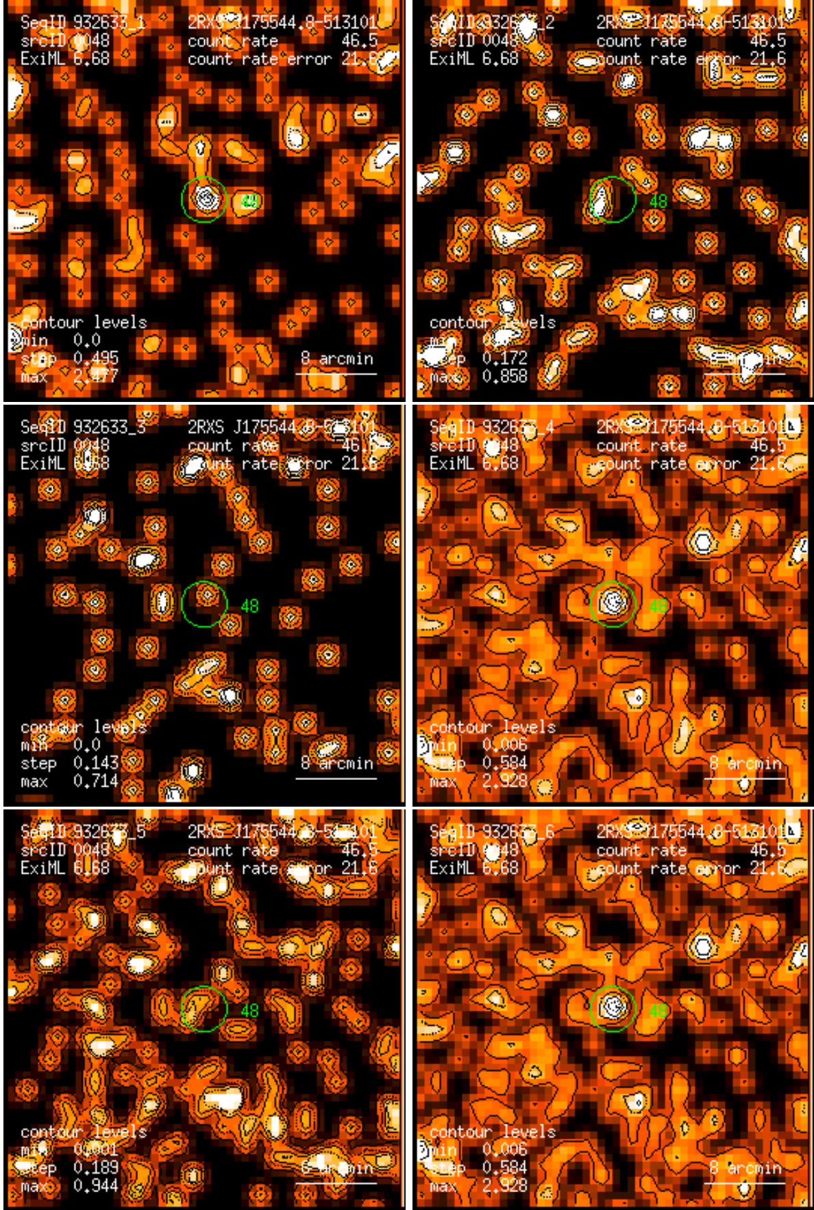
Figure 48: RASS 932633: detection 0048: band rate images, Gaussian filter: (1) PSPC channels 11 – 41, (2) 52 – 90, (3) 91 – 201, (4) 11 – 235, (5) 52 – 201, (6) 11 – 201. Broad band rates in counts/ks. Band rate contour levels in counts/ks/arcmin 2 .
