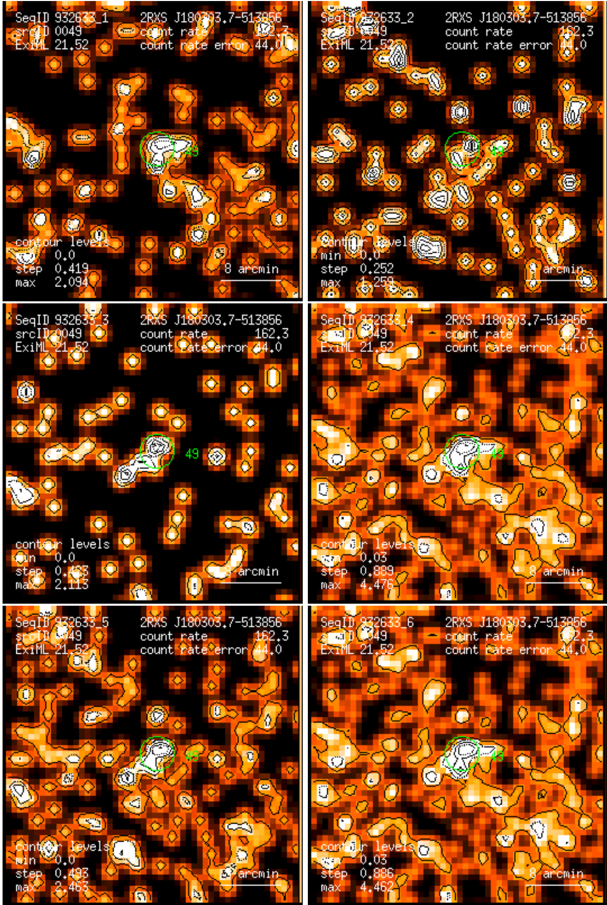
Figure 49: RASS 932633: detection 0049: band rate images, Gaussian filter: (1) PSPC channels 11 – 41, (2) 52 – 90, (3) 91 – 201, (4) 11 – 235, (5) 52 – 201, (6) 11 – 201. Broad band rates in counts/ks. Band rate contour levels in counts/ks/arcmin 2 .
