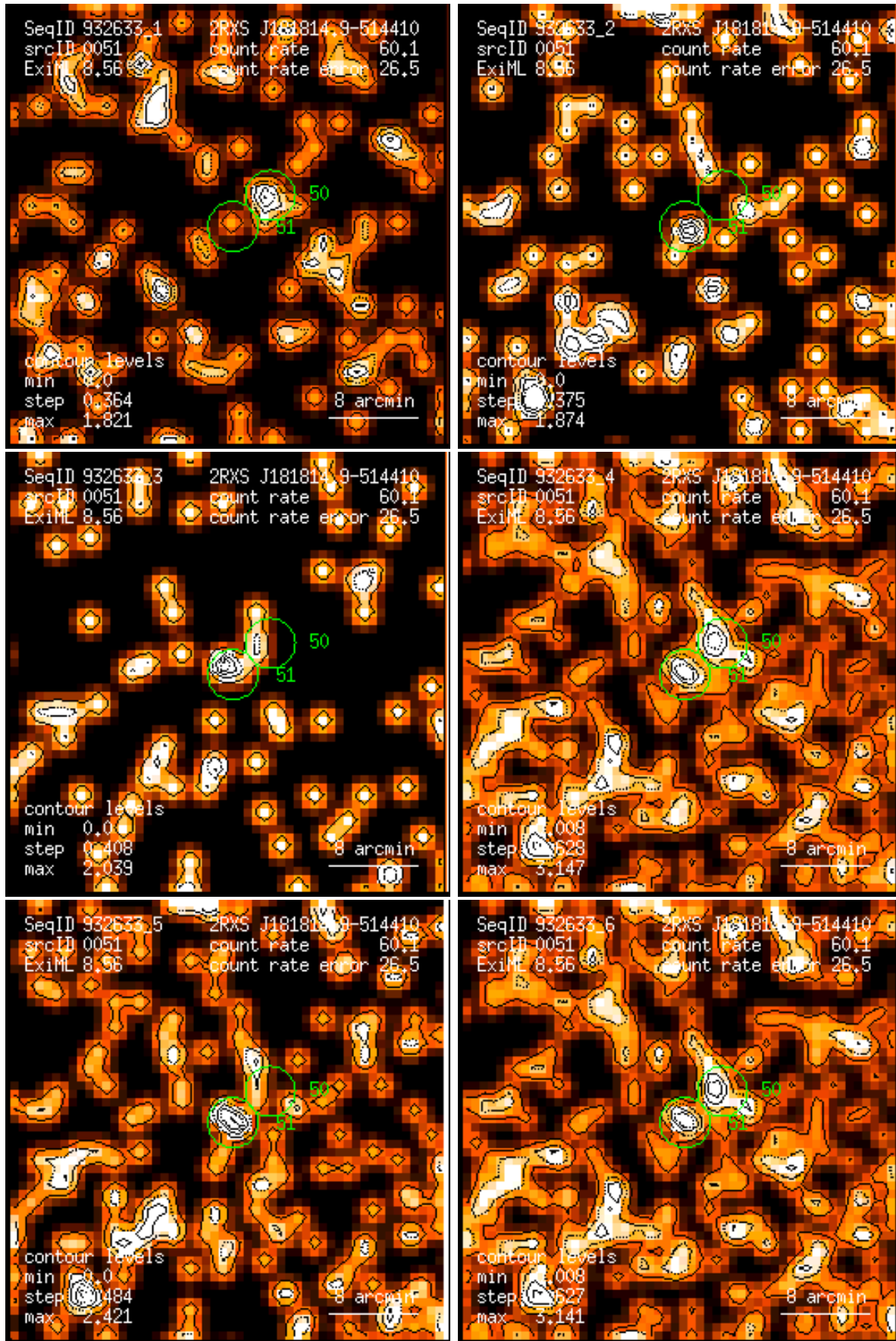
Figure 51: RASS 932633: detection 0051: band rate images, Gaussian filter: (1) PSPC channels 11 – 41, (2) 52 – 90, (3) 91 – 201, (4) 11 – 235, (5) 52 – 201, (6) 11 – 201. Broad band rates in counts/ks. Band rate contour levels in counts/ks/arcmin 2 .
