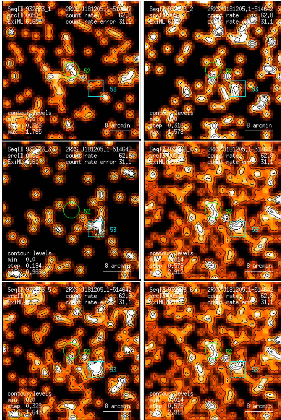
Figure 52: RASS 932633: detection 0052: band rate images, Gaussian filter: (1) PSPC channels 11 – 41, (2) 52 – 90, (3) 91 – 201, (4) 11 – 235, (5) 52 – 201, (6) 11 – 201. Broad band rates in counts/ks. Band rate contour levels in counts/ks/arcmin 2 .
