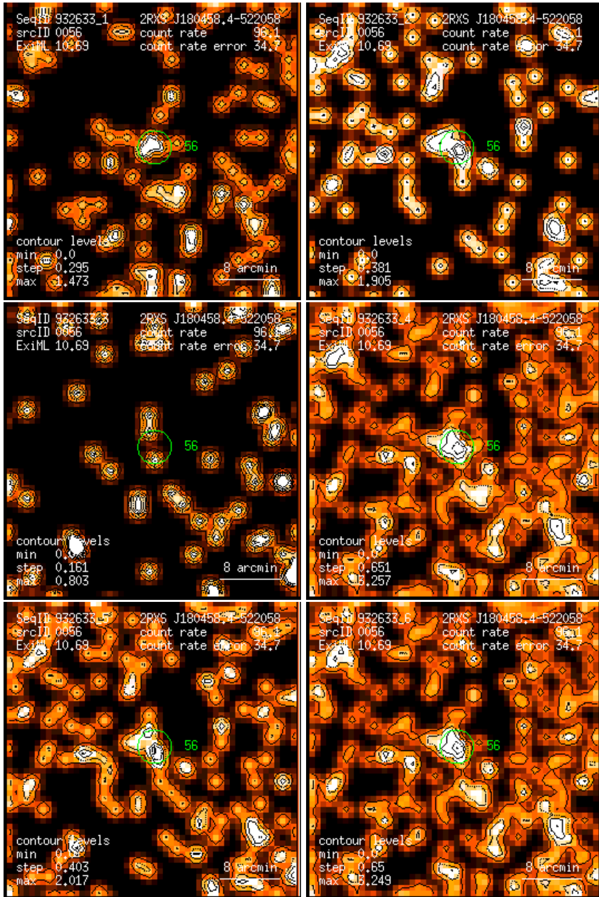
Figure 56: RASS 932633: detection 0056: band rate images, Gaussian filter: (1) PSPC channels 11 – 41, (2) 52 – 90, (3) 91 – 201, (4) 11 – 235, (5) 52 – 201, (6) 11 – 201. Broad band rates in counts/ks. Band rate contour levels in counts/ks/arcmin 2 .
