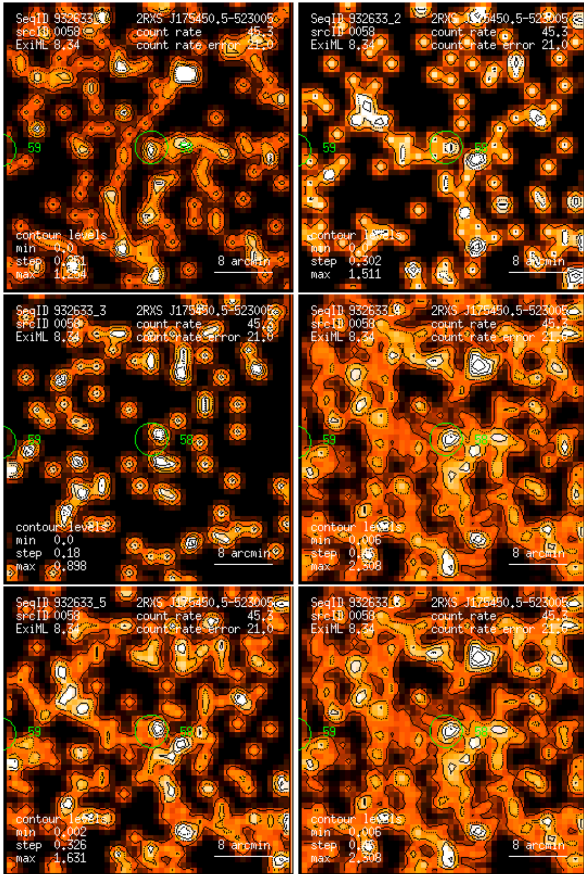
Figure 58: RASS 932633: detection 0058: band rate images, Gaussian filter: (1) PSPC channels 11 – 41, (2) 52 – 90, (3) 91 – 201, (4) 11 – 235, (5) 52 – 201, (6) 11 – 201. Broad band rates in counts/ks. Band rate contour levels in counts/ks/arcmin 2 .
