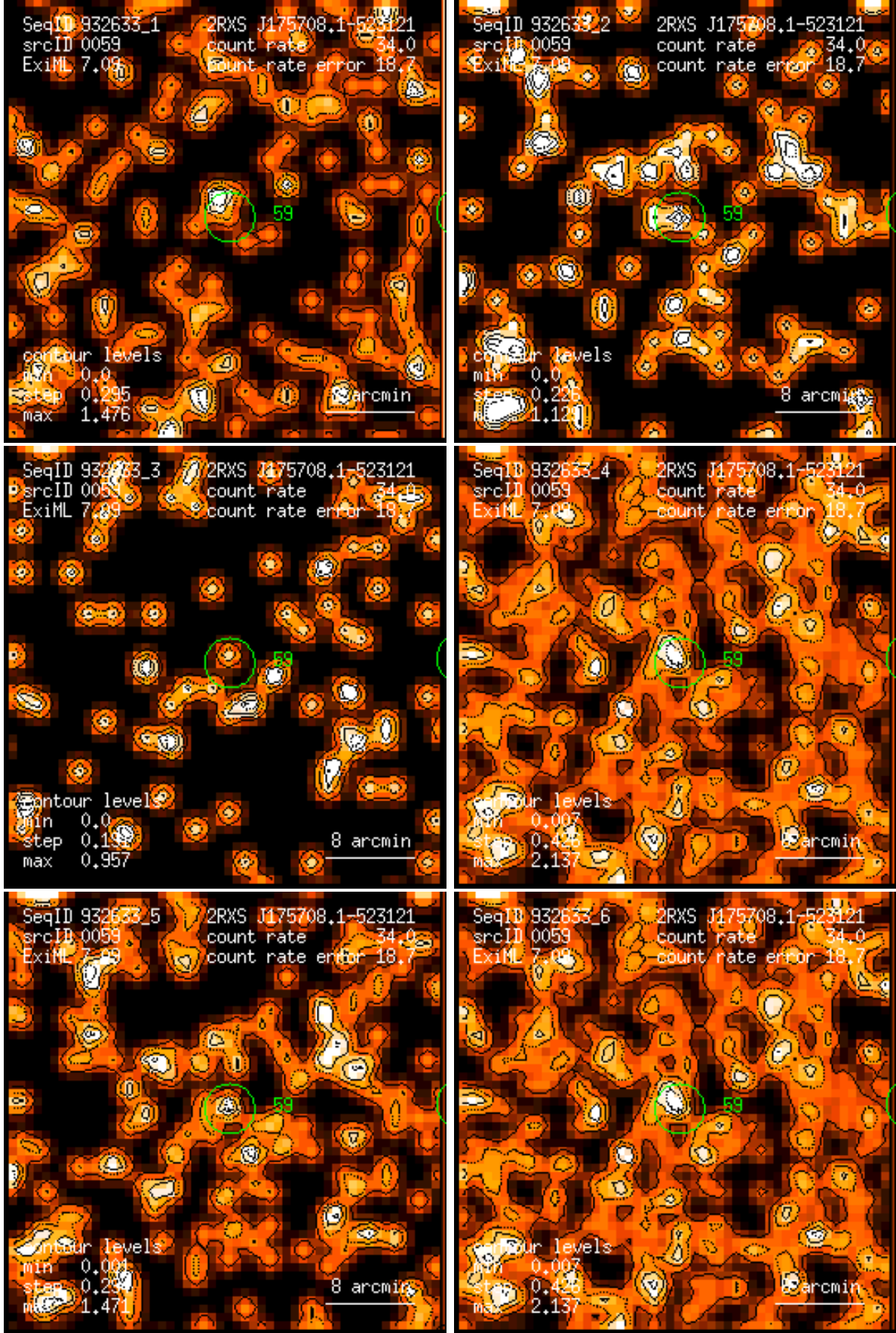
Figure 59: RASS 932633: detection 0059: band rate images, Gaussian filter: (1) PSPC channels 11 – 41, (2) 52 – 90, (3) 91 – 201, (4) 11 – 235, (5) 52 – 201, (6) 11 – 201. Broad band rates in counts/ks. Band rate contour levels in counts/ks/arcmin 2 .
